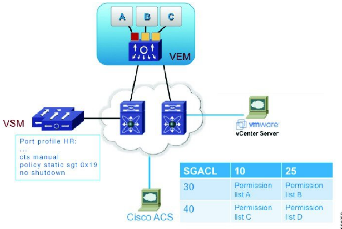
Figure 3: SGT and SGACL in Cisco TrustSec Network
