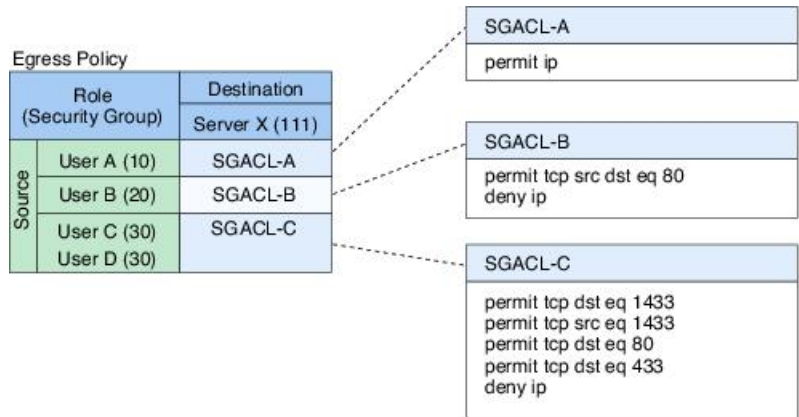
Figure 4: SGACL Policy Matrix Example
