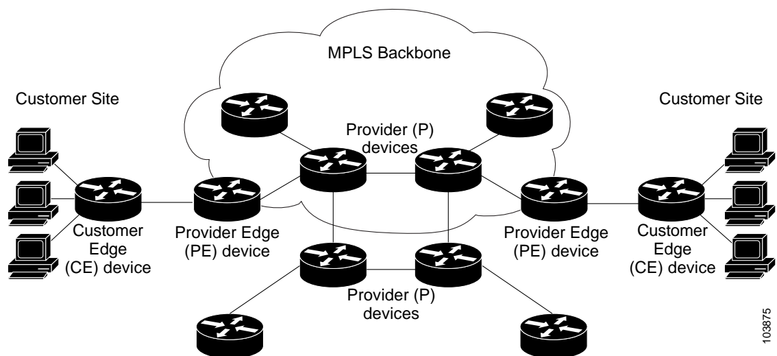
Figure 20-1 Basic MPLS Layer 3 VPN Terminology
