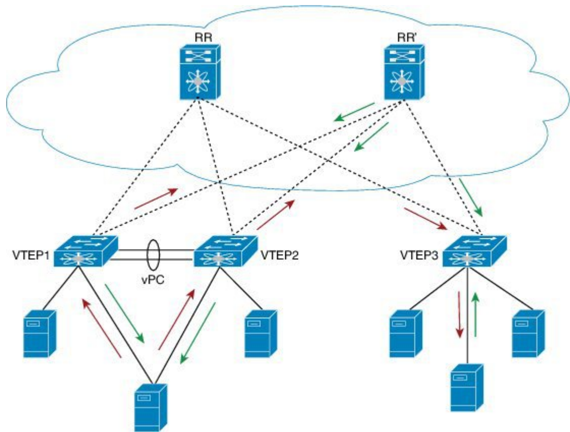
Figure 2: vPC configuration
