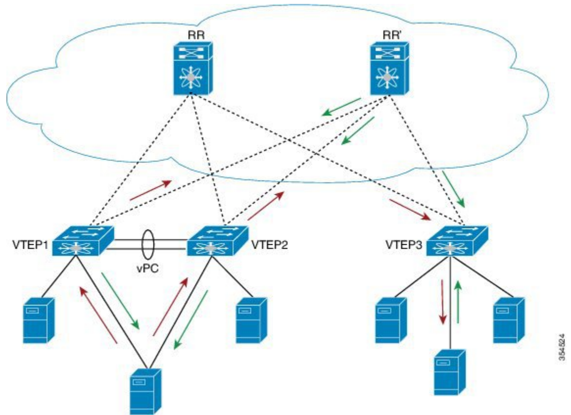
Figure 1: vPC configuration
