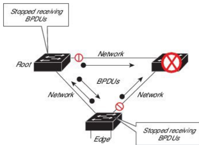
Figure 12: Network Problem Averted with Bridge Assurance Enabled
