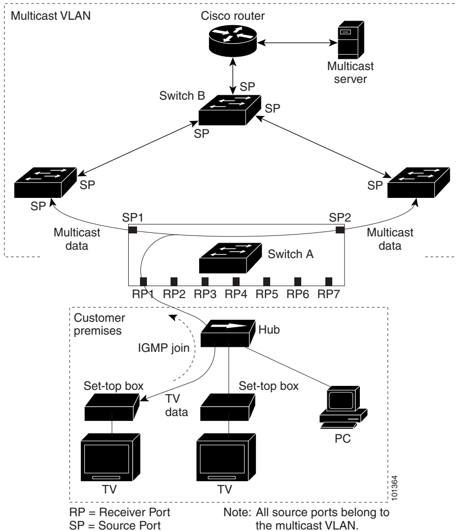
Figure 27-3 Multicast VLAN Registration Example
