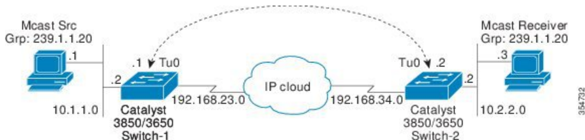
Figure 15: Tunnel Connecting Non-IP Multicast Areas
