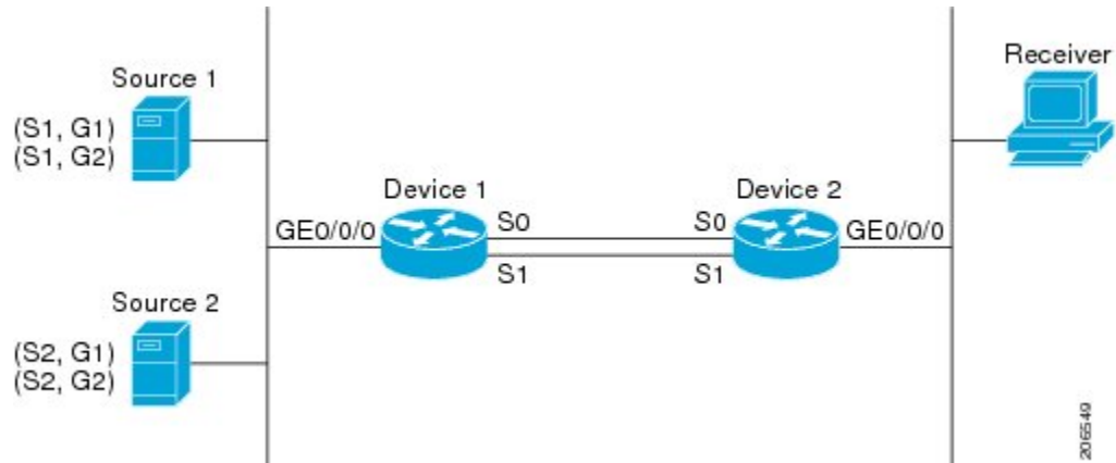
Figure 18: Default Behavior for IP Multicast When Multiple Equal-Cost Paths Exist
