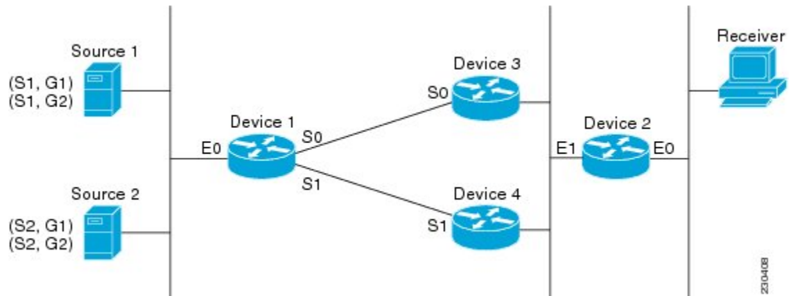
Figure 20: ECMP Multicast Load Splitting and Assert Processing in PIM-DM and DF Election in Bidir-PIM
