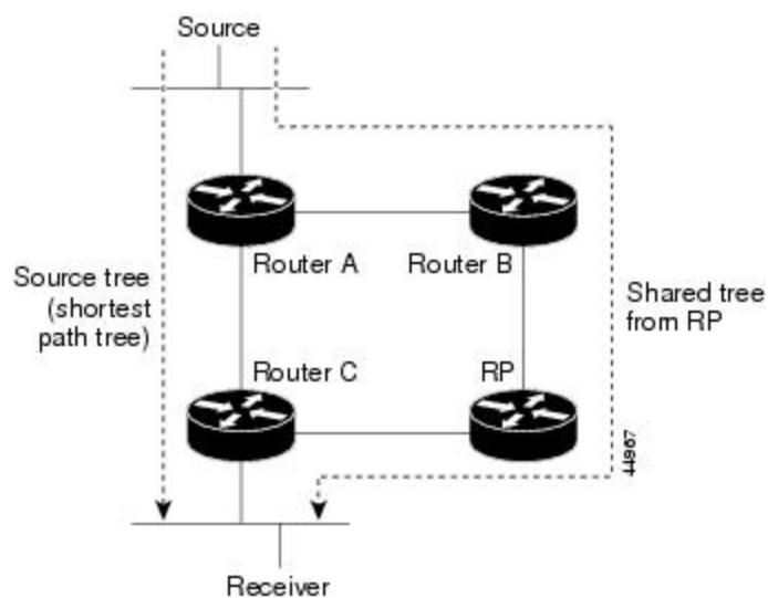
Figure 7: Shared Tree and Source Tree (Shortest-Path Tree)
