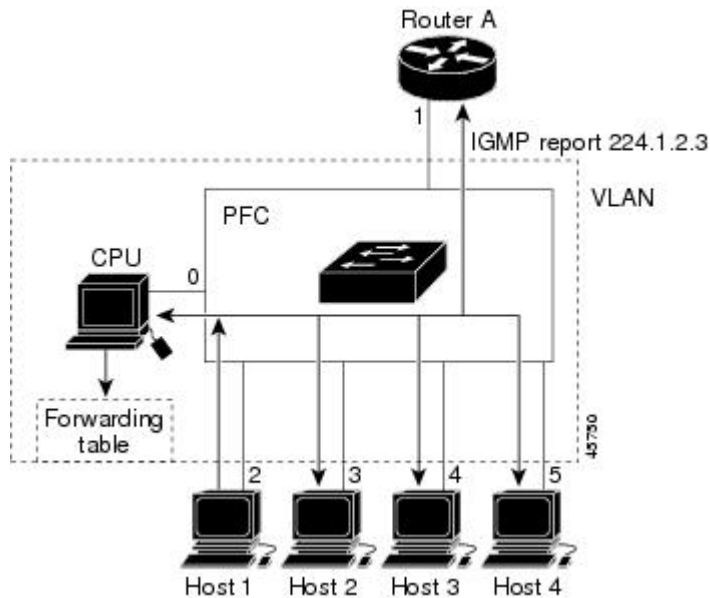
Figure 3: Initial IGMP Join Message
