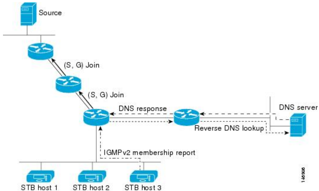
Figure 14: DNS-Based SSM Mapping
