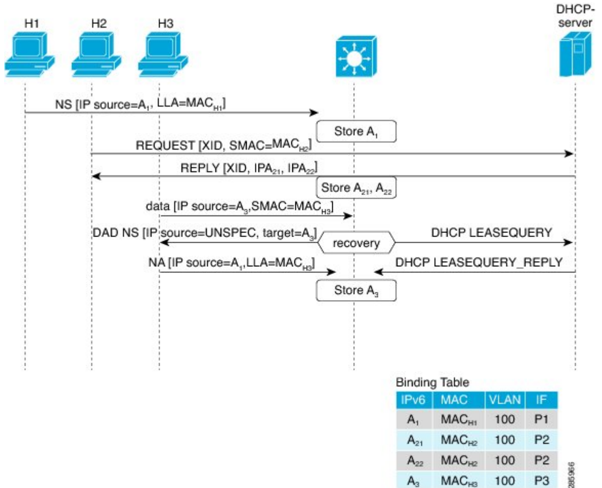
Figure 13: IPv6 Address Glean
