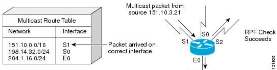
Figure 9: RPF Check Succeeds
