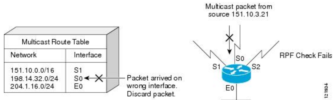
Figure 8: RPF Check Fails
