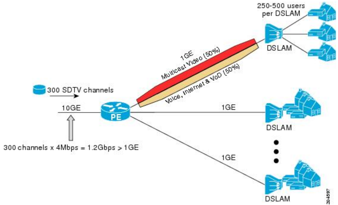
Figure 22: IGMP State Limit Example Topology
