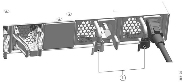
Figure 9: AC-Power Supply with Velcro Strap
