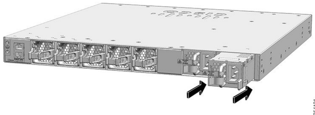
Figure 7: Inserting the AC-Power Supply in the Catalyst WS-C3850-48XS Switch
