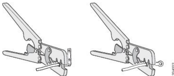
Figure 11: Crimping the Ground Lug
