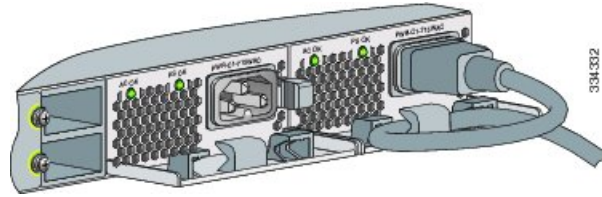
Figure 9: AC-Power Supply with Velcro Strap
