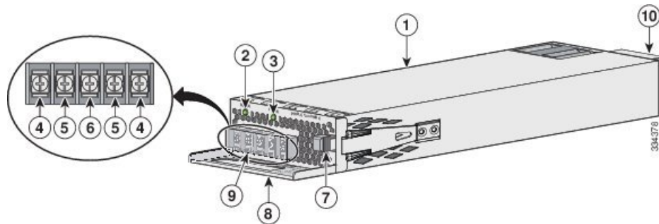
Figure 4: 440-W DC Power Supply
