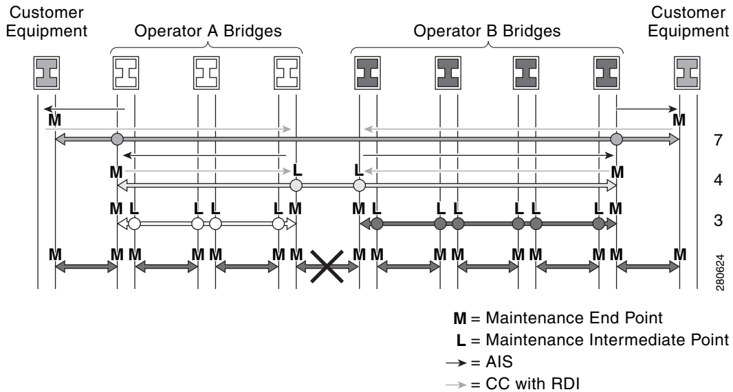
Figure 54-1 Generating and Propagating AIS Messages Upon a Defect (Link Fail)
