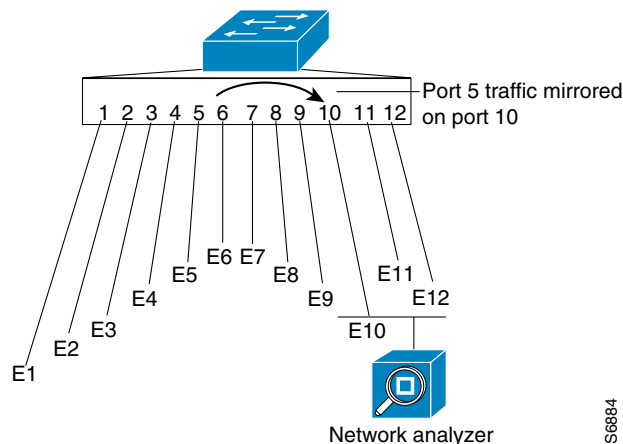
Figure 49-1 Example SPAN Configuration
