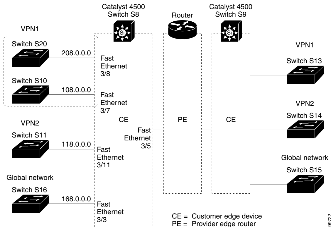
Figure 35-2 VRF-lite Configuration Example
