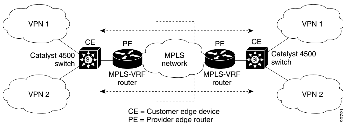
Figure 35-1 Catalyst 4500 Series Switches Acting as Multiple Virtual CEs
