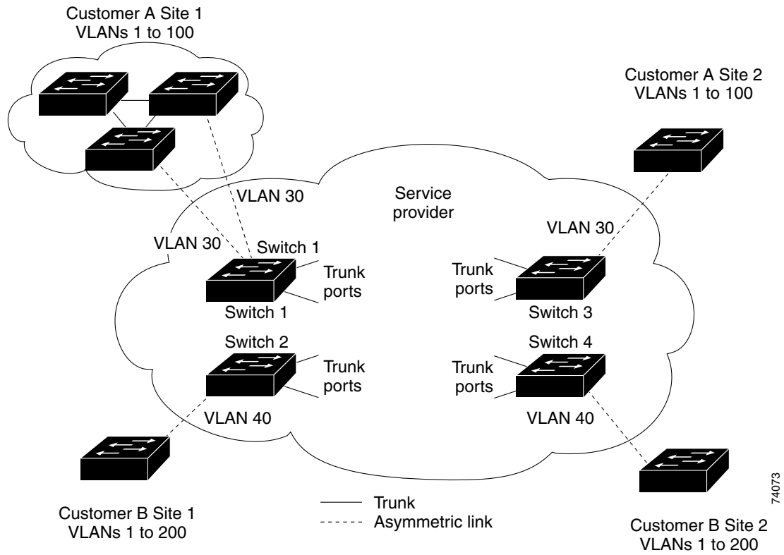
Figure 25-4 Layer 2 Protocol Tunneling
