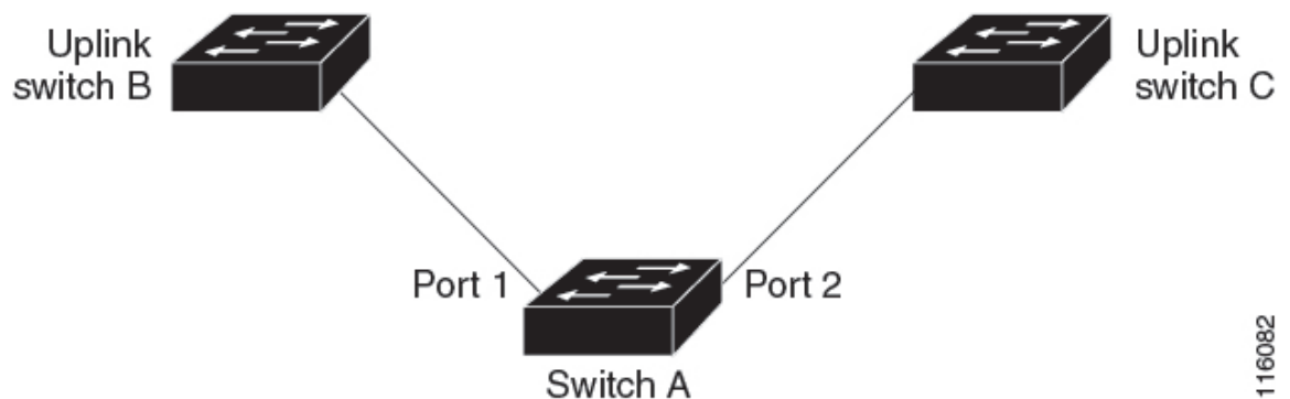
Figure 35: FlexLink+ Topology
