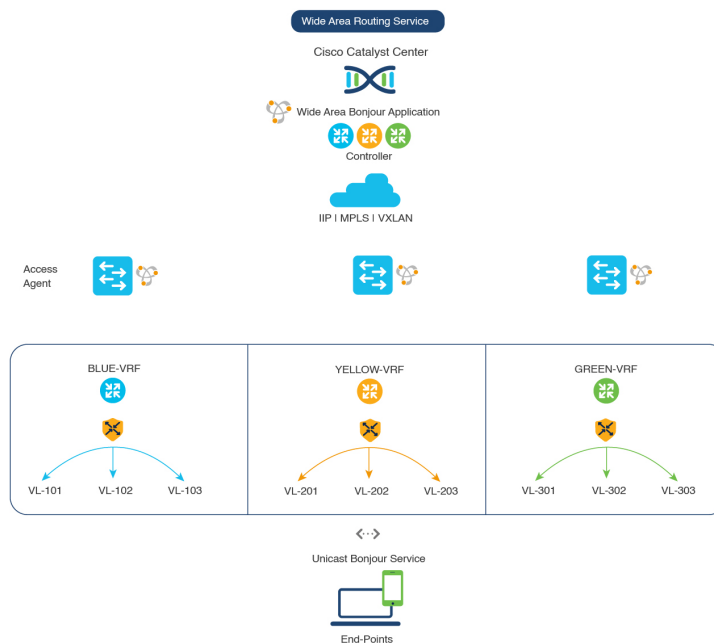
Figure 3: VRF-Aware Wide Area Bonjour Services
