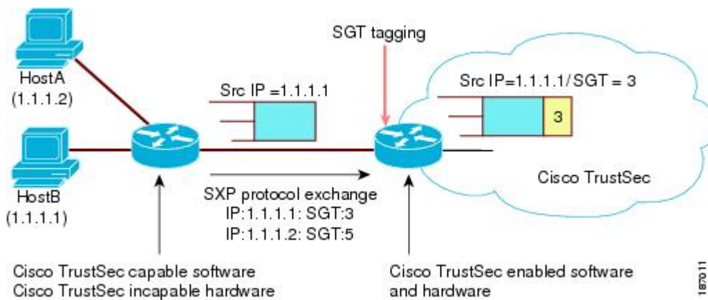
Figure 5: SXP Protocol to Propagate SGT Information
