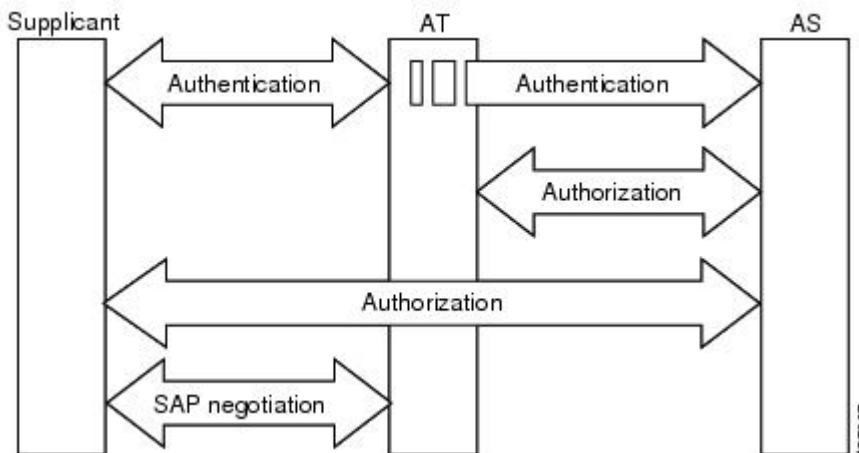
Figure 4: NDAC and SAP Negotiation
