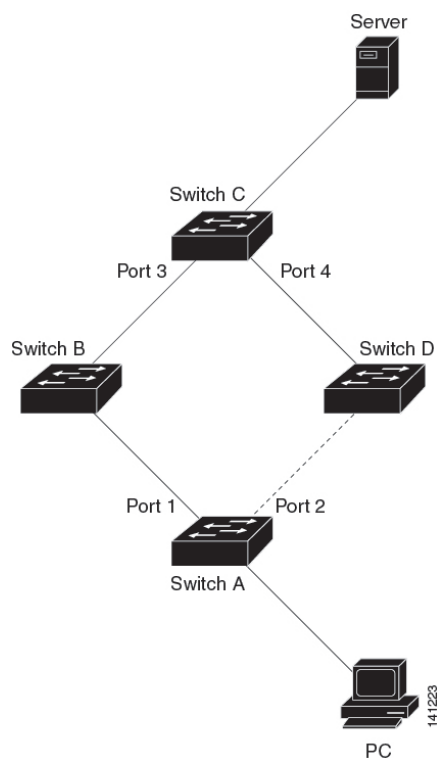
Figure 34: Transmission of Dummy Multicast Packets in FlexLink+ Topology
