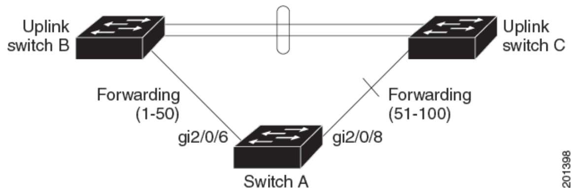
Figure 33: VLAN Load Balancing in FlexLink+ Topology
