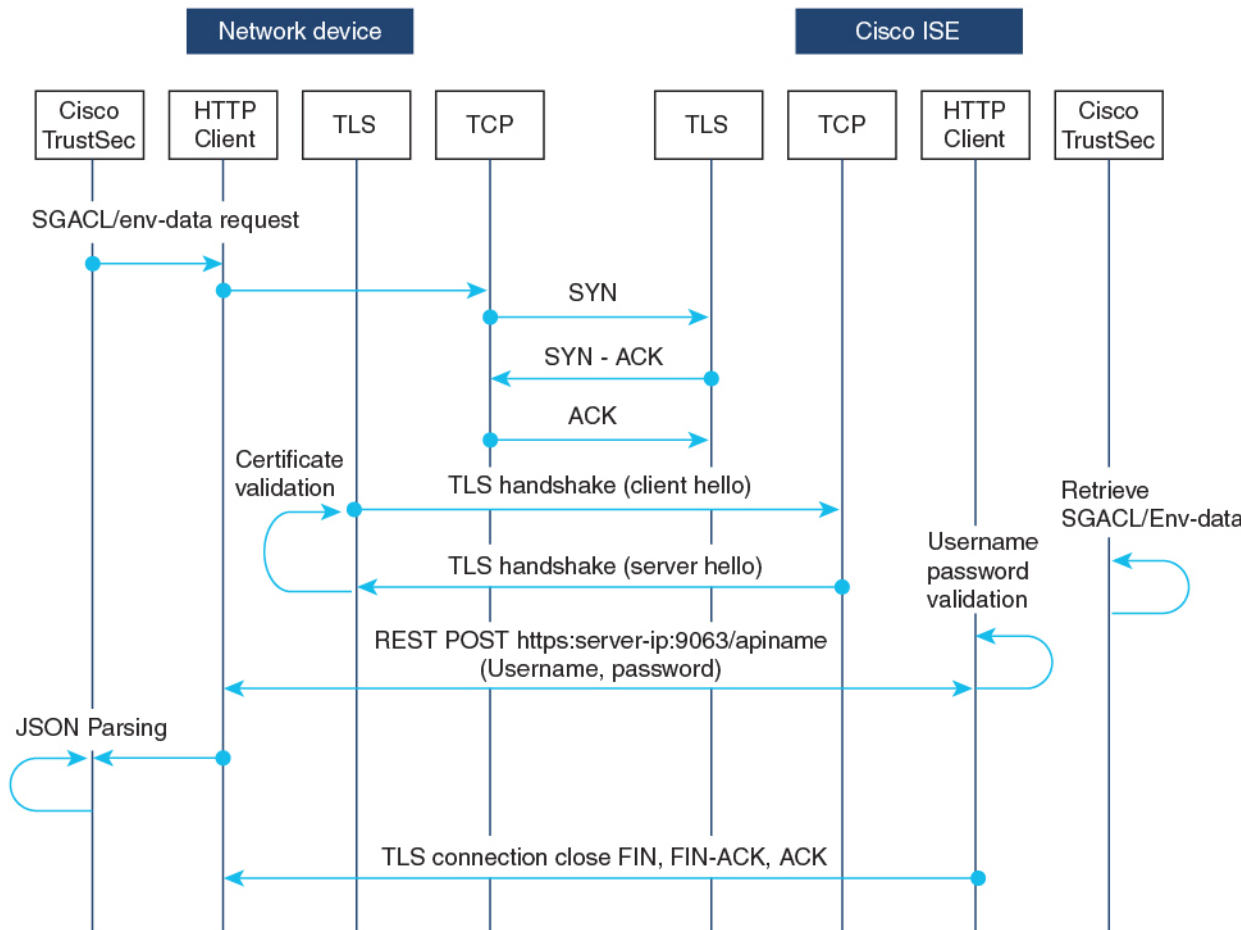
Figure 7: Message Flow Between a Network Device and a Server
