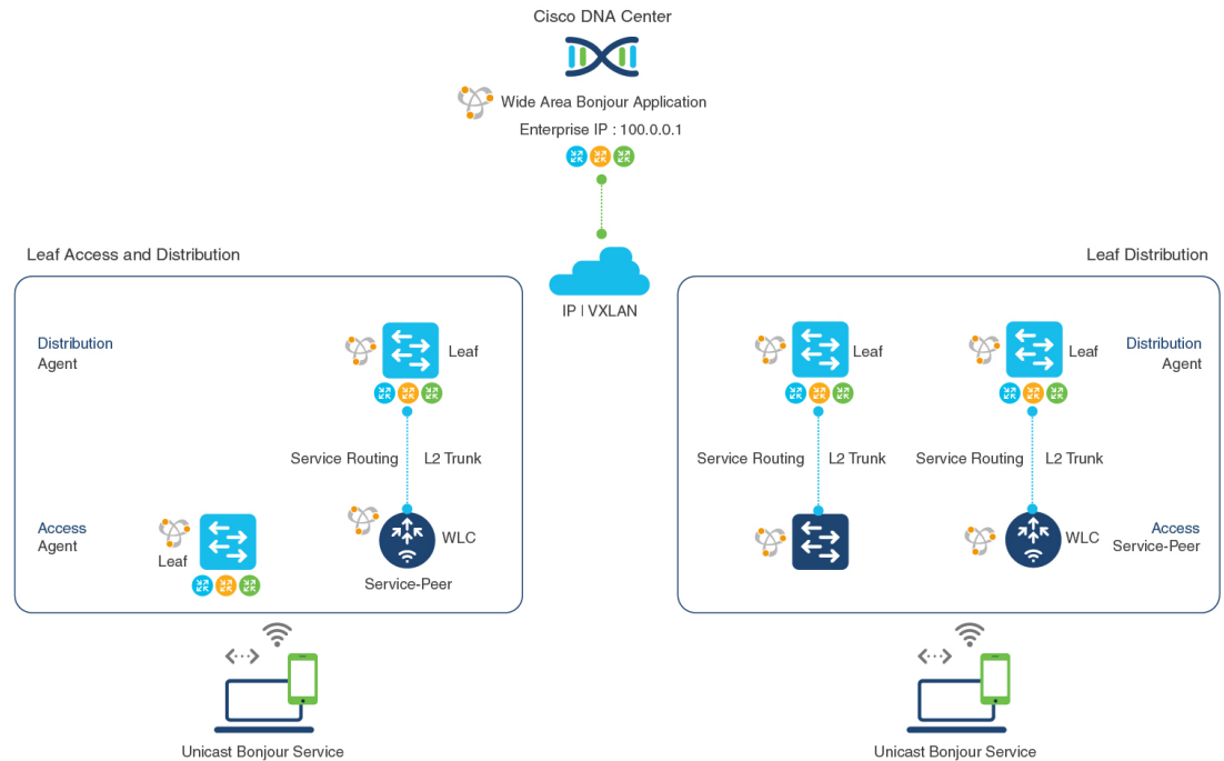
Figure 7: Deployment Model for Wide Area Bonjour over BGP EVPN VXLAN
