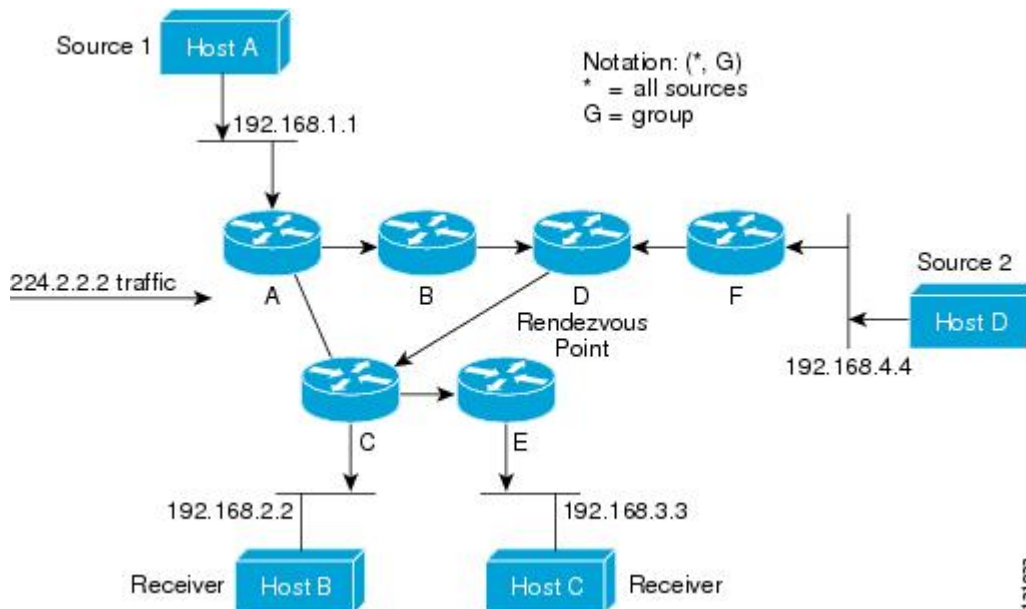
Figure 5: Shared Tree
