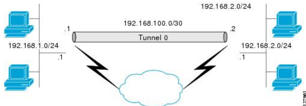
Figure 48: IPsec SVTI
