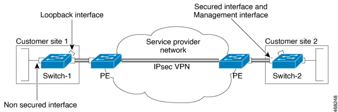
Figure 46: IPsec Network
