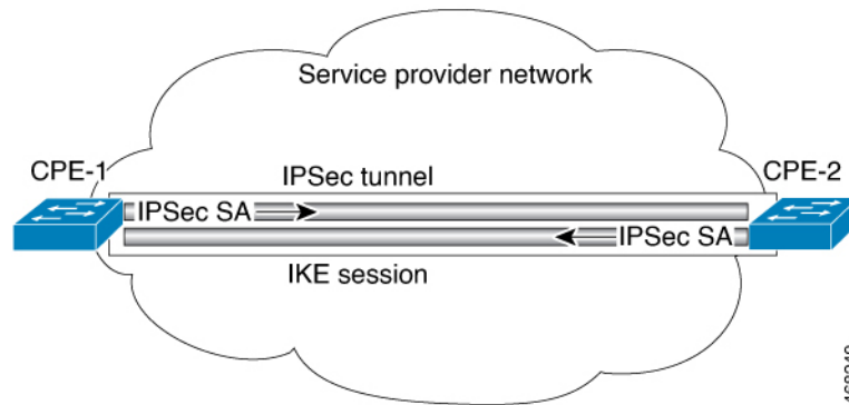
Figure 47: IPsec Tunnel
