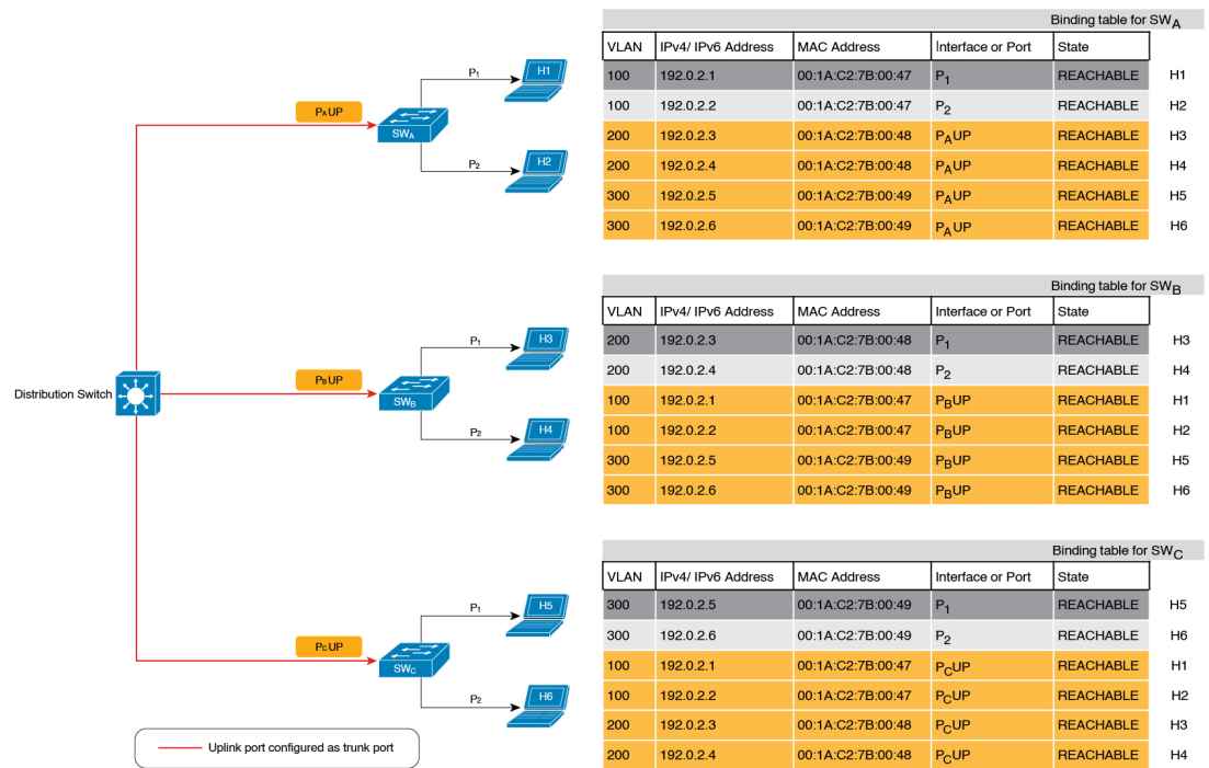
Figure 27: Multi-Switch Set-Ups Without Trusted-Port and Device-Role Switch Options
