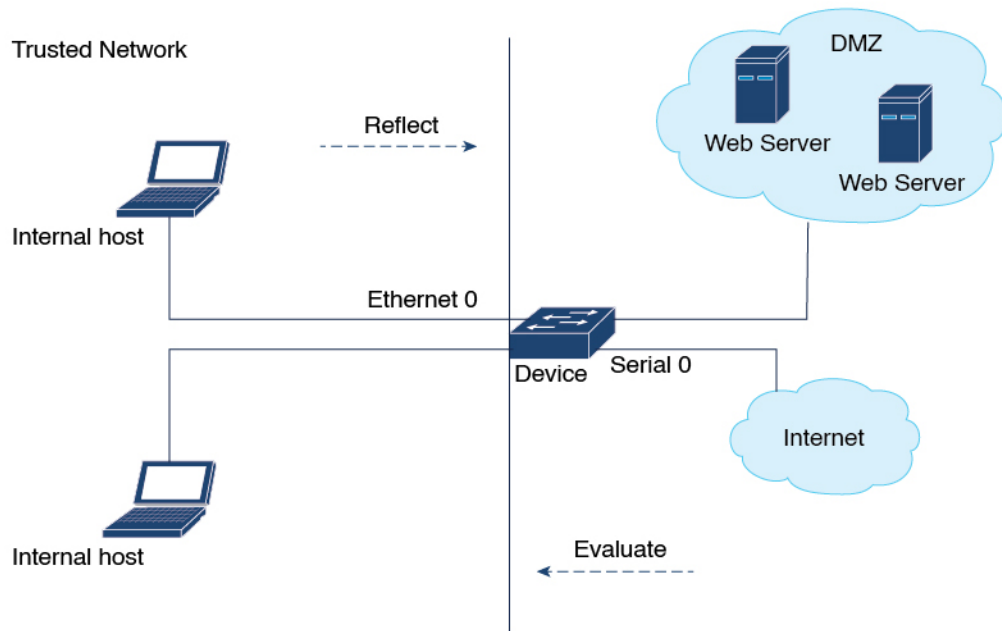
Figure 19: Reflexive Access List for the Internal Interface
