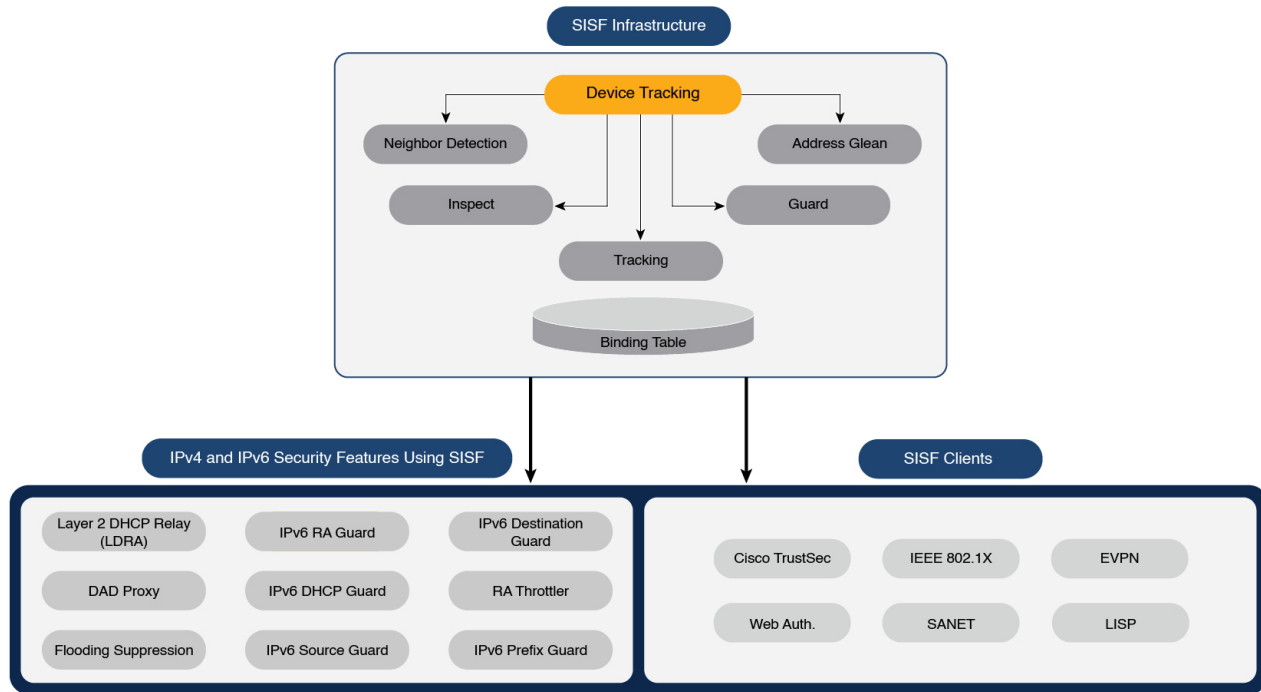
Figure 22: SISF Framework
