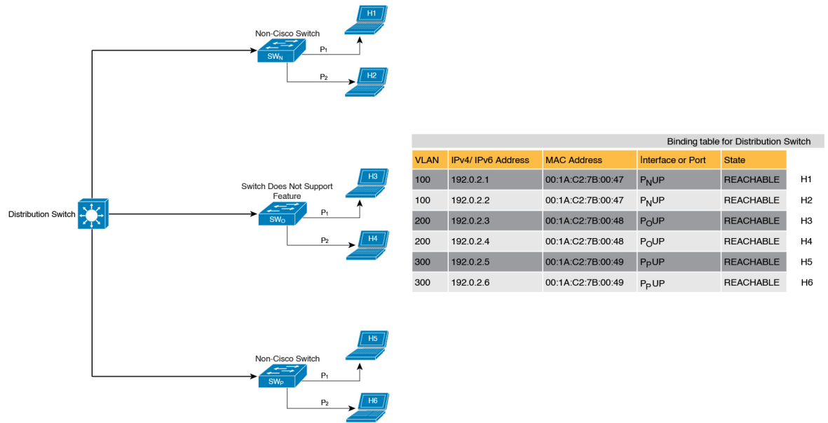
Figure 29: Centralised Binding Table
