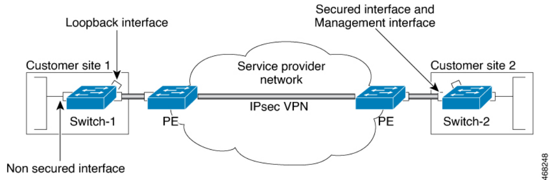
Figure 1: IPsec Network
