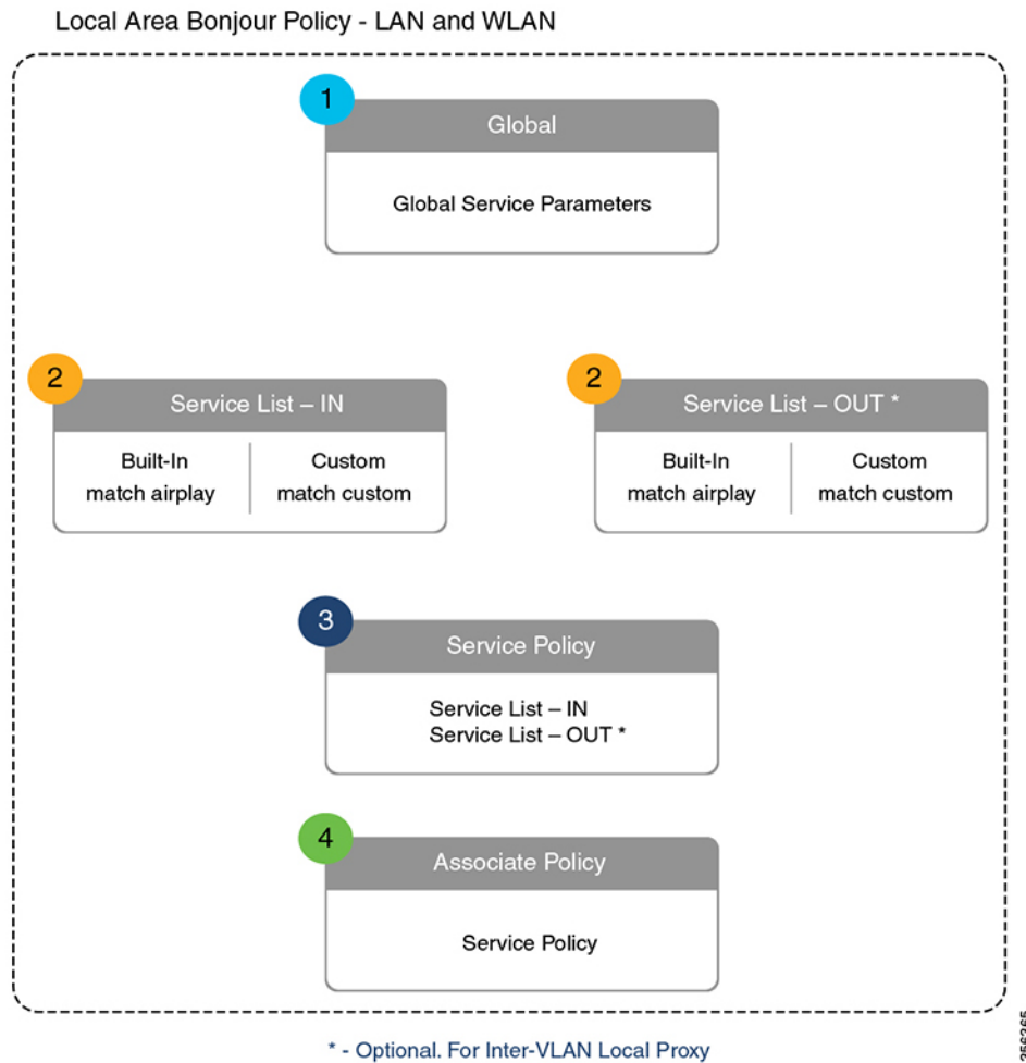
Figure 22: Local Area Bonjour Policy Hierarchy
