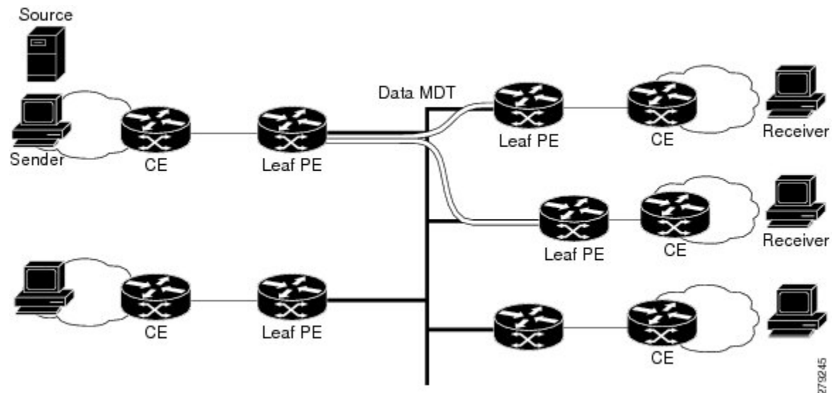
Figure 33: MLDP with the Data MDT Scenario
