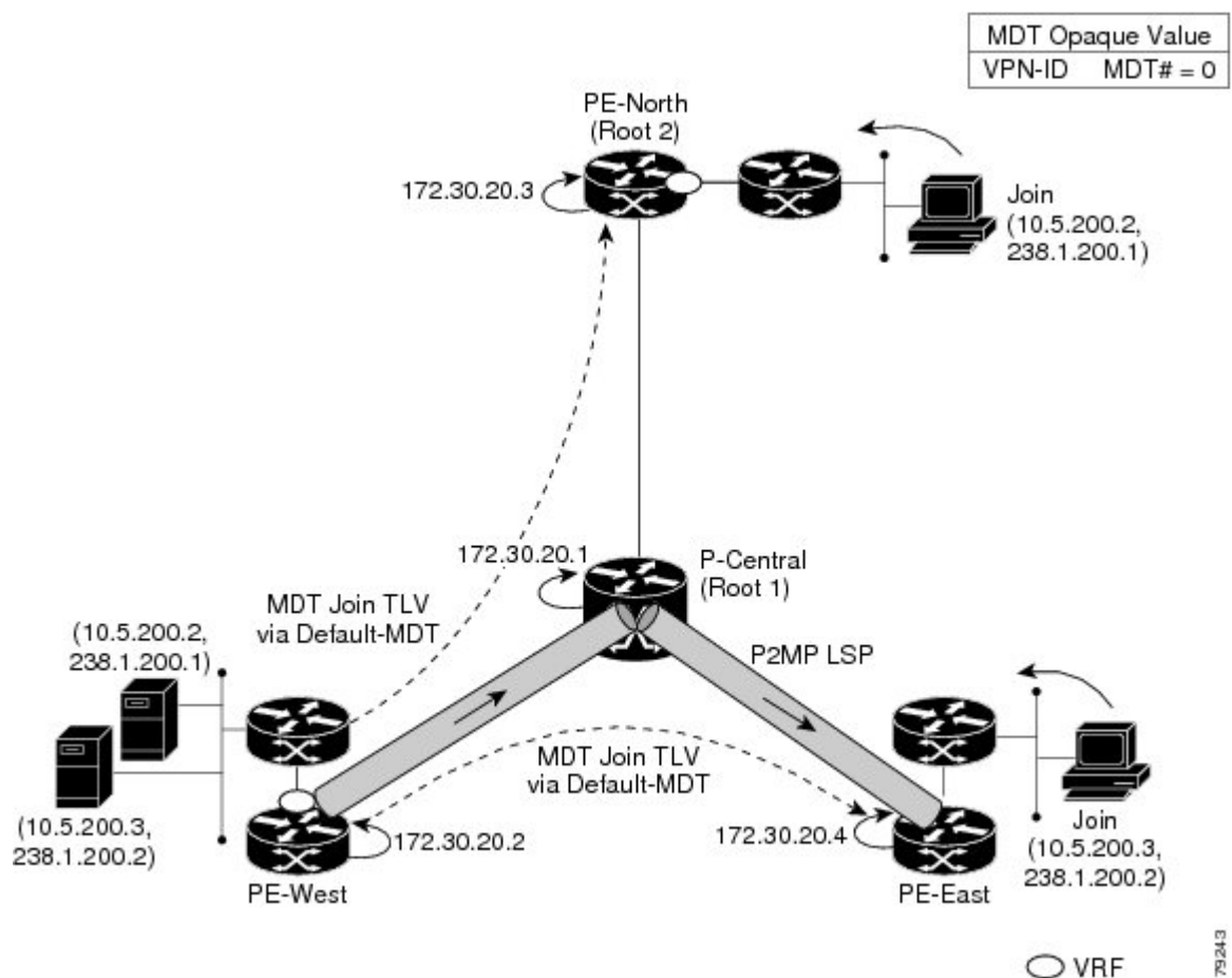
Figure 42: Data MDT Example
