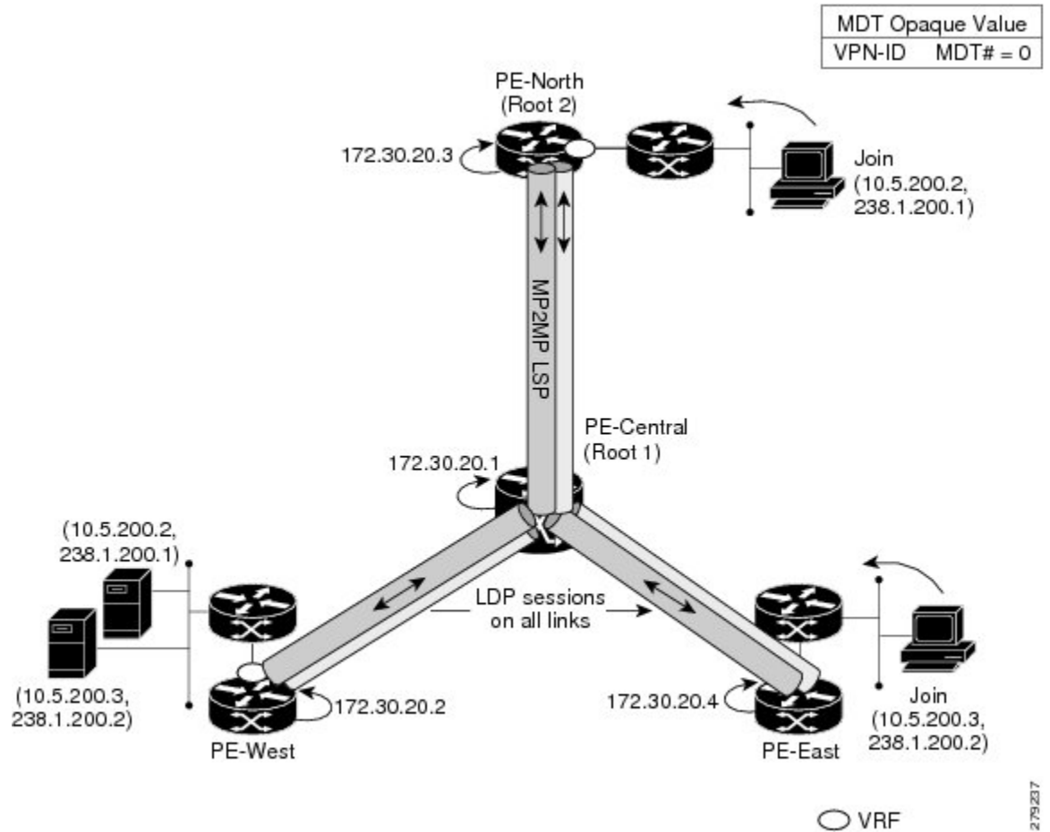
Figure 34: Default MDT Scenario
