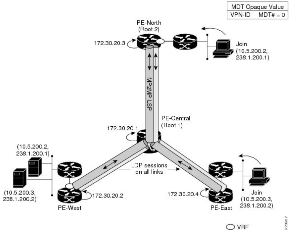
Figure 41: Default MDT Example
