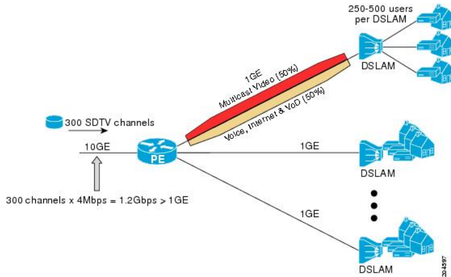
Figure 47: IGMP State Limit Example Topology
