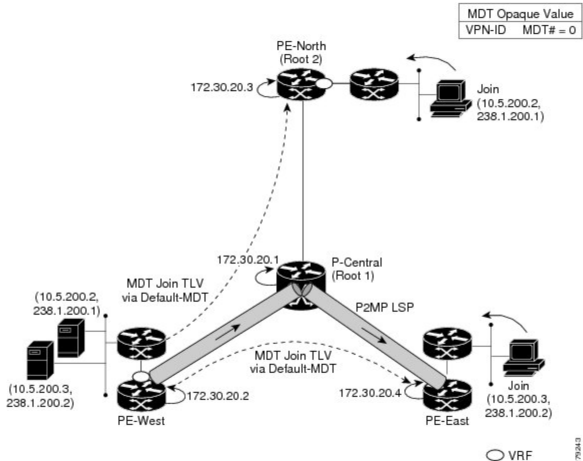
Figure 40: Data MDT Scenario
