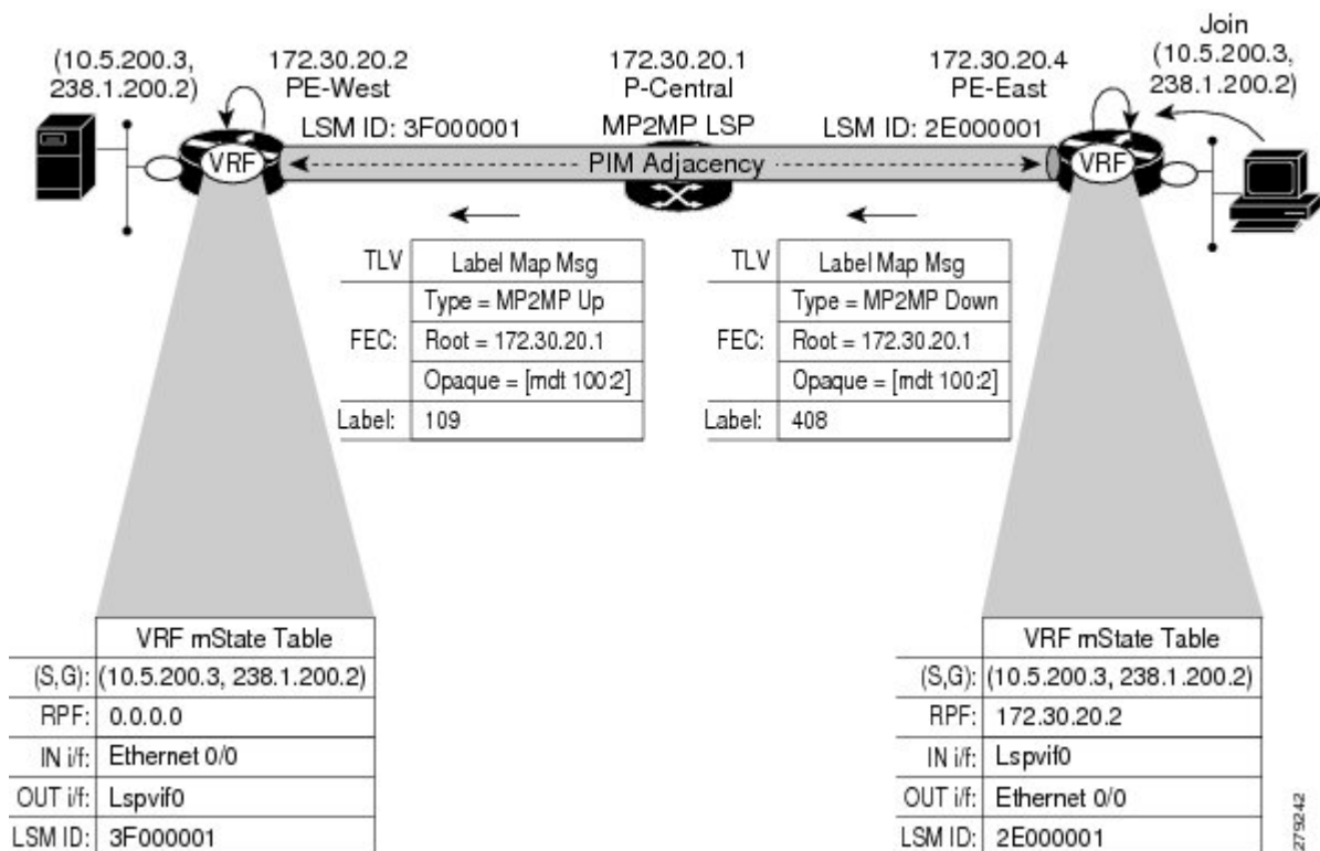
Figure 39: PIM Signaling over LSP
