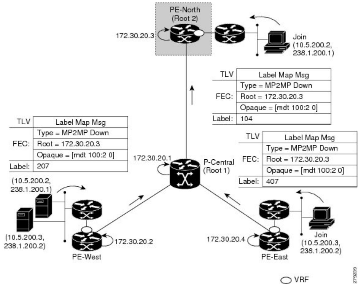
Figure 36: Default MDT Downstream--Root 2
