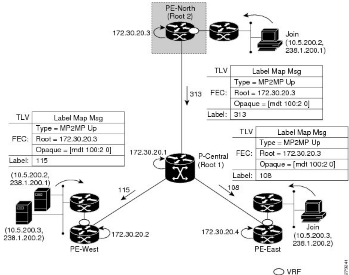
Figure 38: Default MDT Upstream--Root 2
