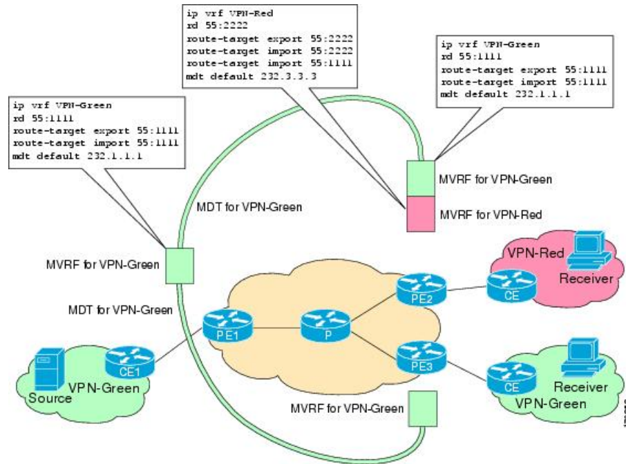
Figure 30: Topology for mVPN Extranet Support Option 1 Configuration Example
