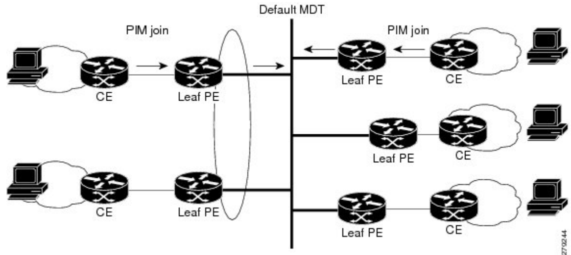
Figure 32: MLDP with the Default MDT Scenario
