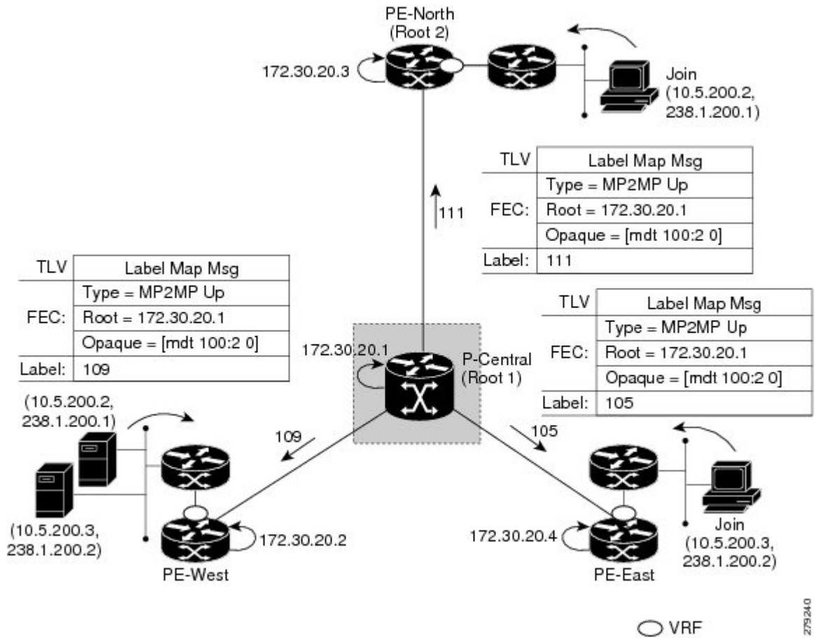
Figure 37: Default MDT Upstream--Root 1
