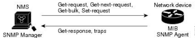
Figure 2: SNMP Network
