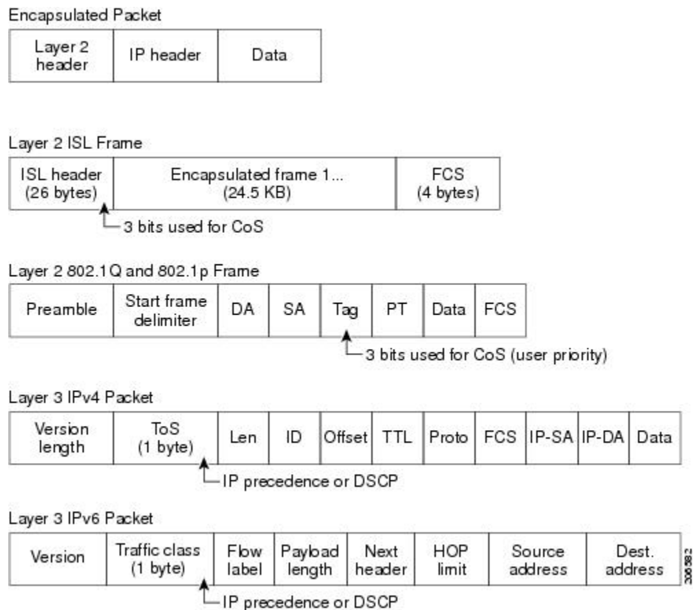
Figure 1: Classification Layers of QoS in Frames and Packets
