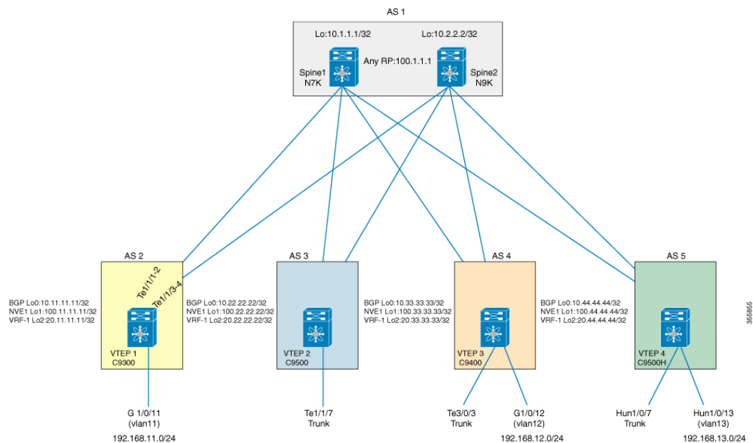
Figure 29: shows the topology used in the eBGP Multi-AS design model
