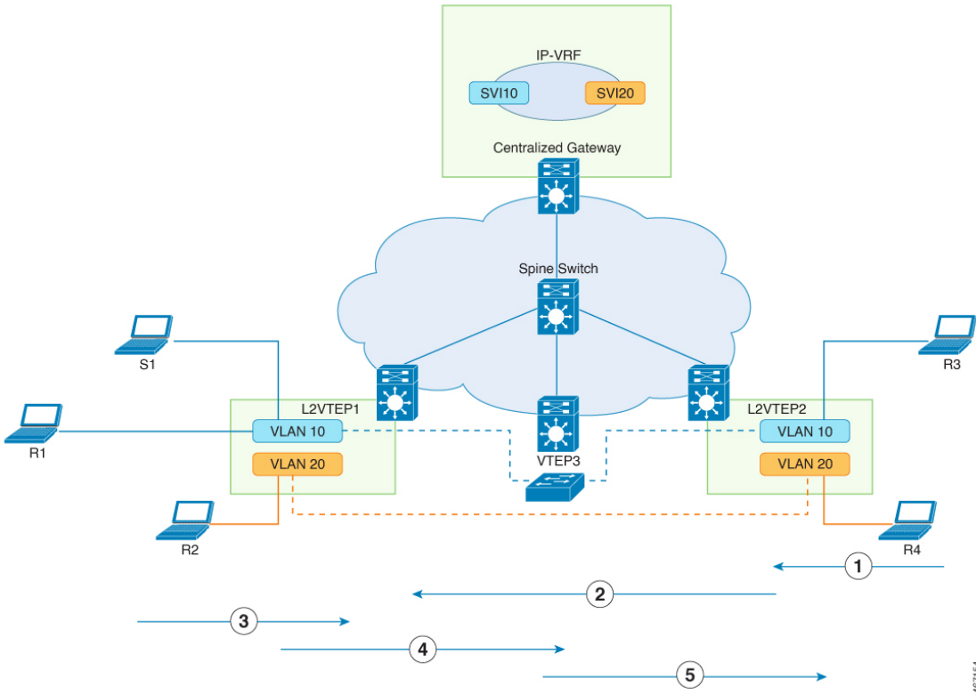
Figure 62: Topology to show Layer 2 Overlay Multicast Traffic within a VLAN
