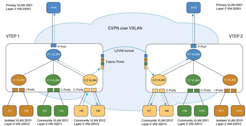
Figure 60: BUM Traffic from Community Port (H5)
