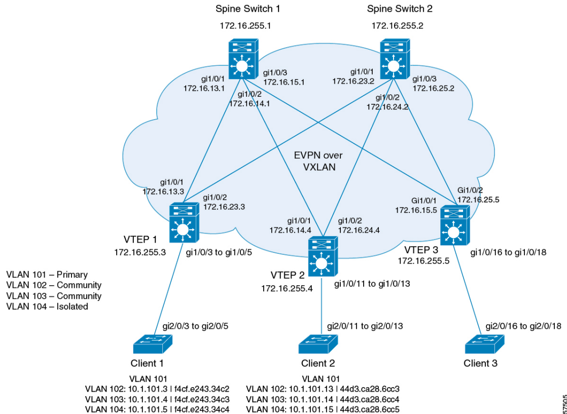
Figure 61: Private VLANs in a BGP EVPN VXLAN Fabric
