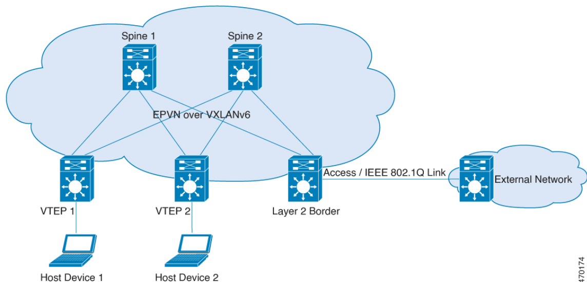
Figure 71: EVPN VXLANv6 Fabric with Layer 2 Gateway
