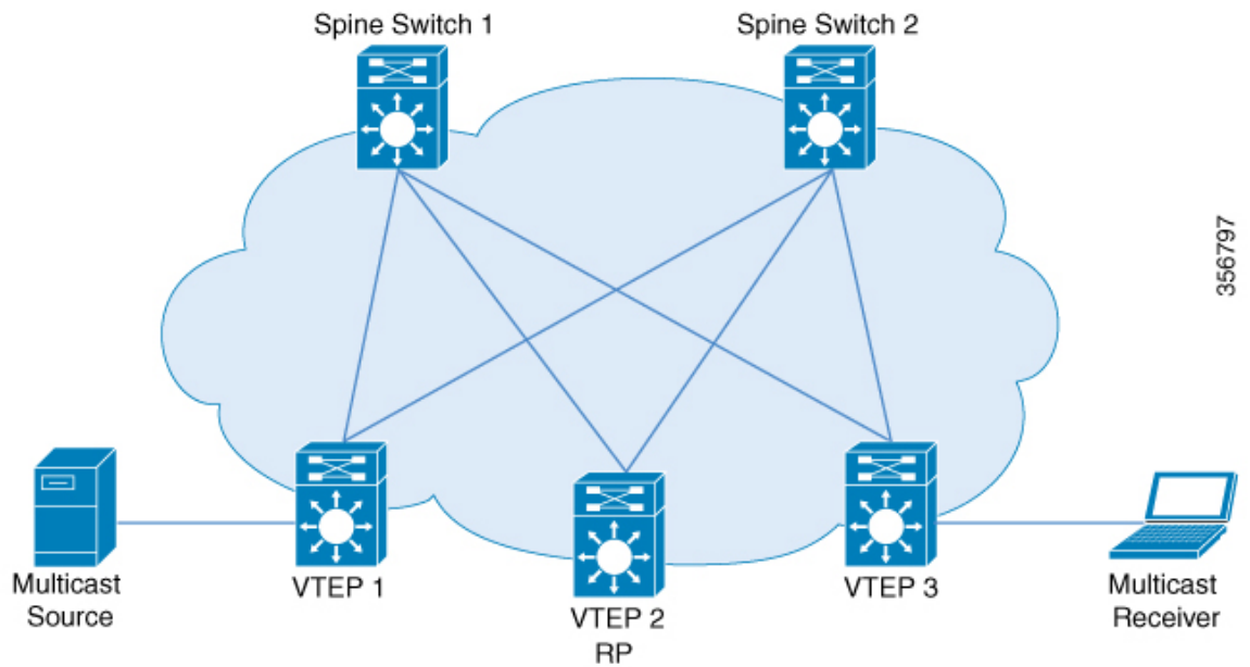
Figure 31: VTEP as an RP
