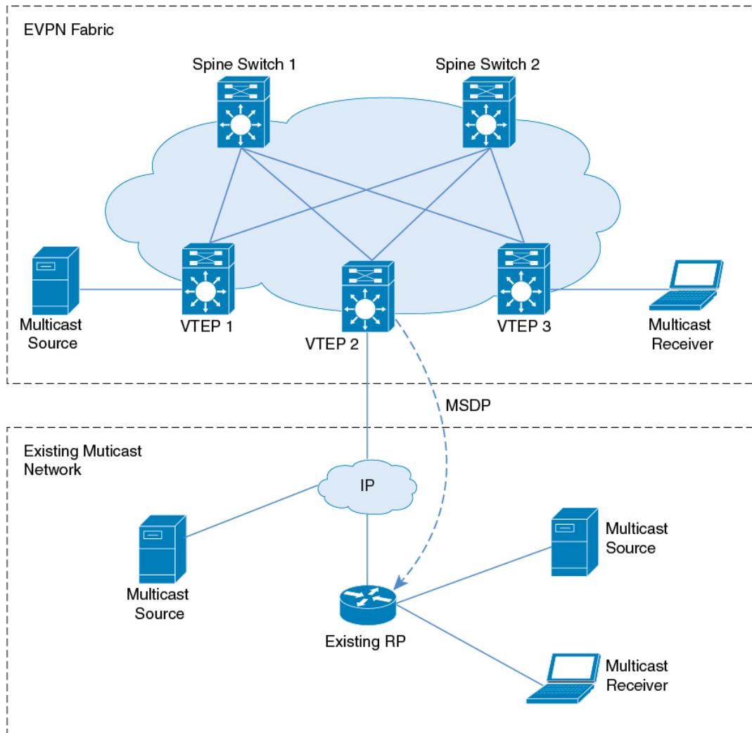
Figure 29: Anycast RP with IPv4 Overlay in an Existing Multicast Network
