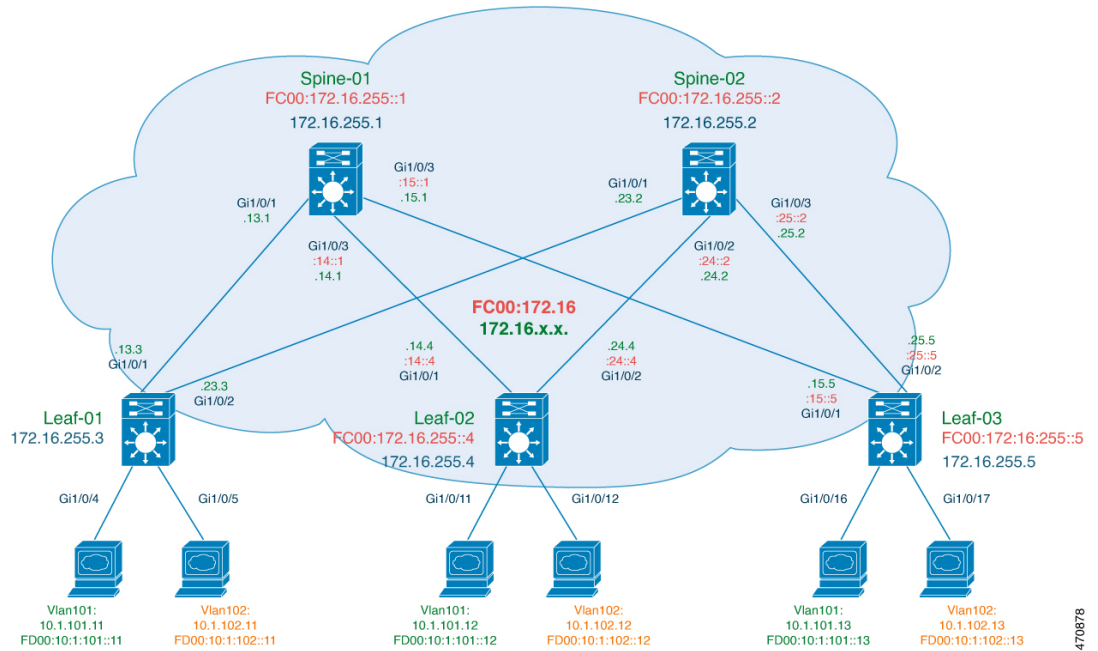
Figure 74: BGP EVPN VXLAN with a Dual Stack Underlay
