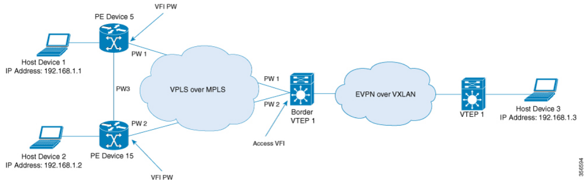
Figure 45: Layer 2 External Connectivity with a VPLS Network Through an Access VFI
