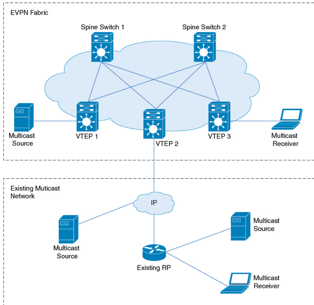
Figure 32: RP Outside the BGP EVPN VXLAN Fabric with an Existing Multicast Network
