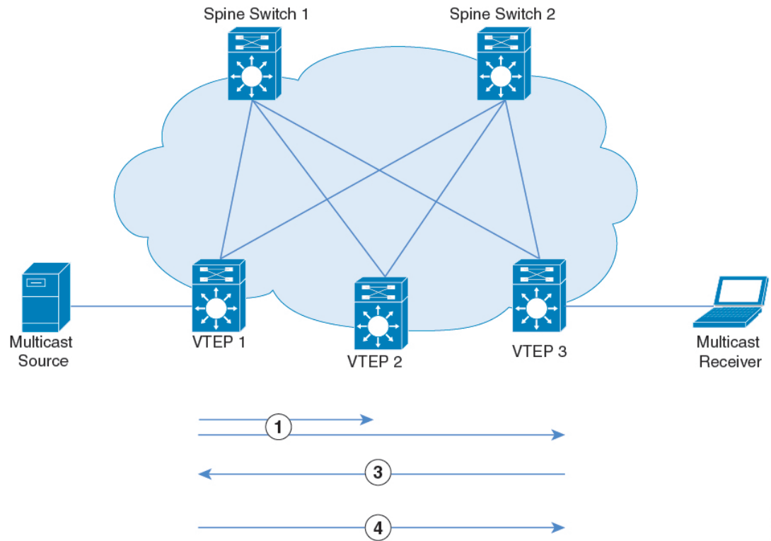
Figure 37: Data MDT Mode
