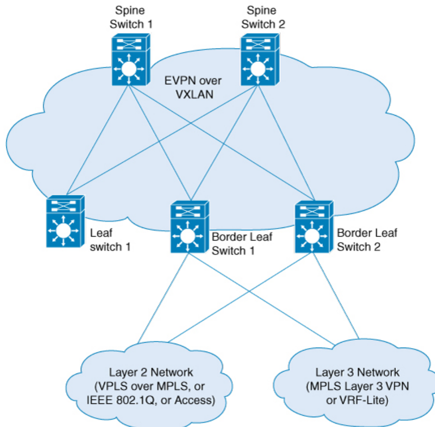
Figure 40: EVPN VXLAN External Connectivity Through a Border Leaf Switch
