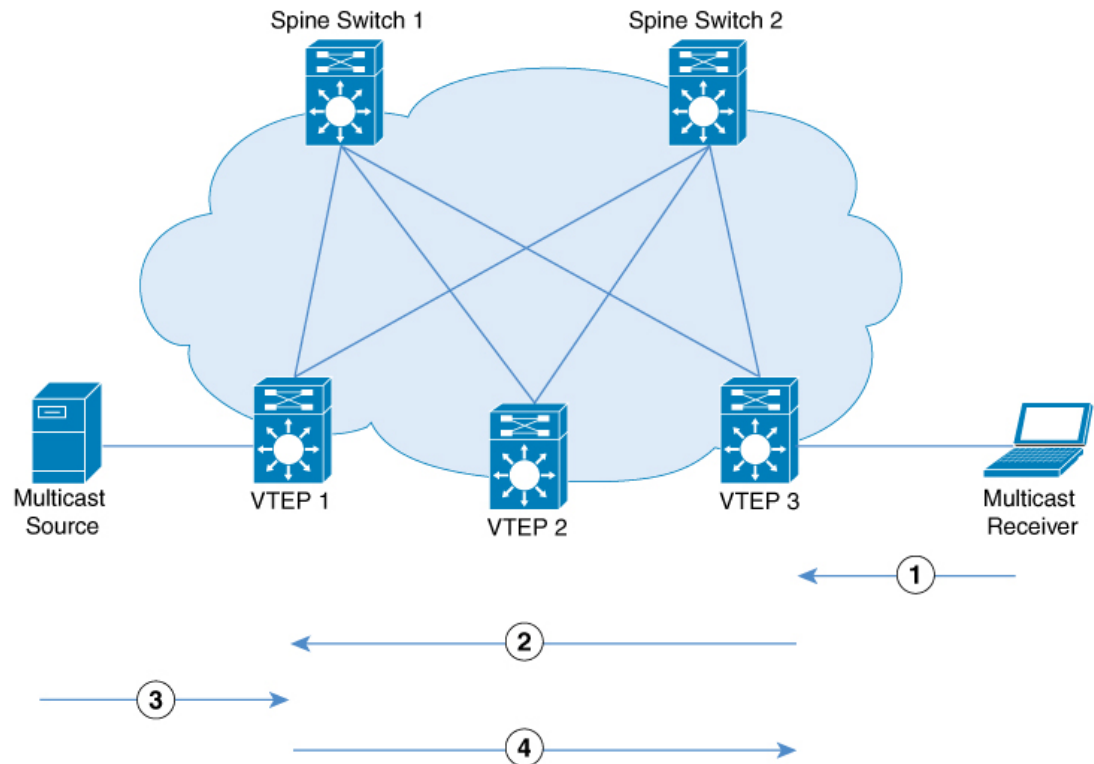
Figure 36: PIM Source Specific Mode
