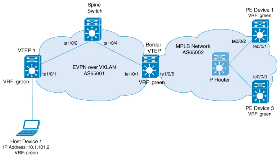
Figure 47: Layer 3 External Connectivity with MPLS Layer 3 VPN through eBGP
