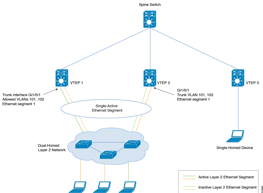
Figure 50: Dual-Homed Network Topology
