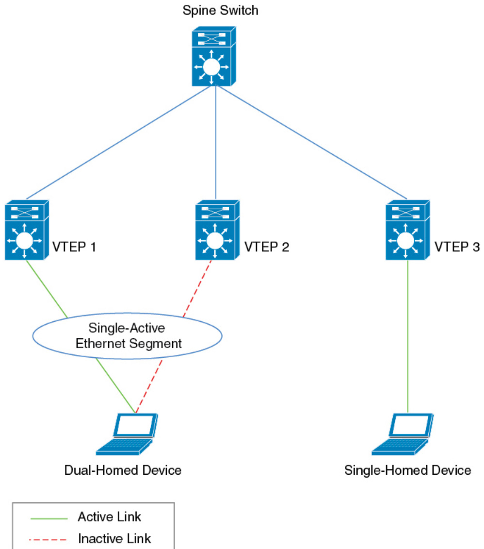
Figure 49: Dual-Homed Device Topology
