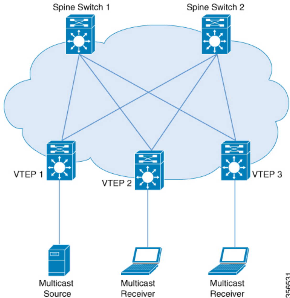
Figure 27: Tenant Routed Multicast Topology
