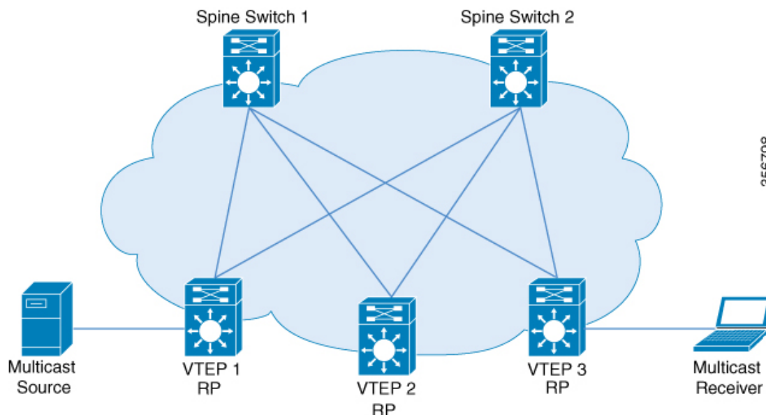
Figure 28: Anycast RP in the Overlay Network
