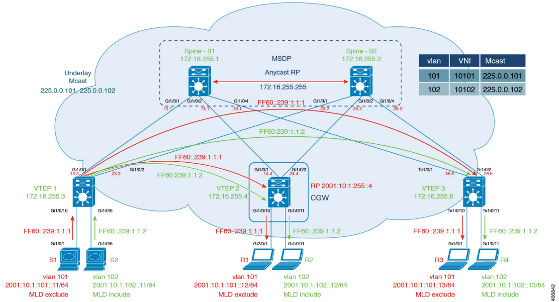
Figure 68: Topology for Optimized Layer 2 Overlay Multicast for IPv6 with Underlay Multicast Replication
