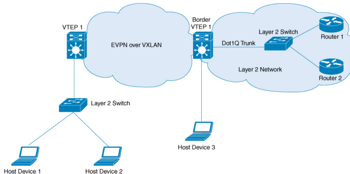
Figure 44: Layer 2 External Connectivity with IEEE 802.1Q Networks
