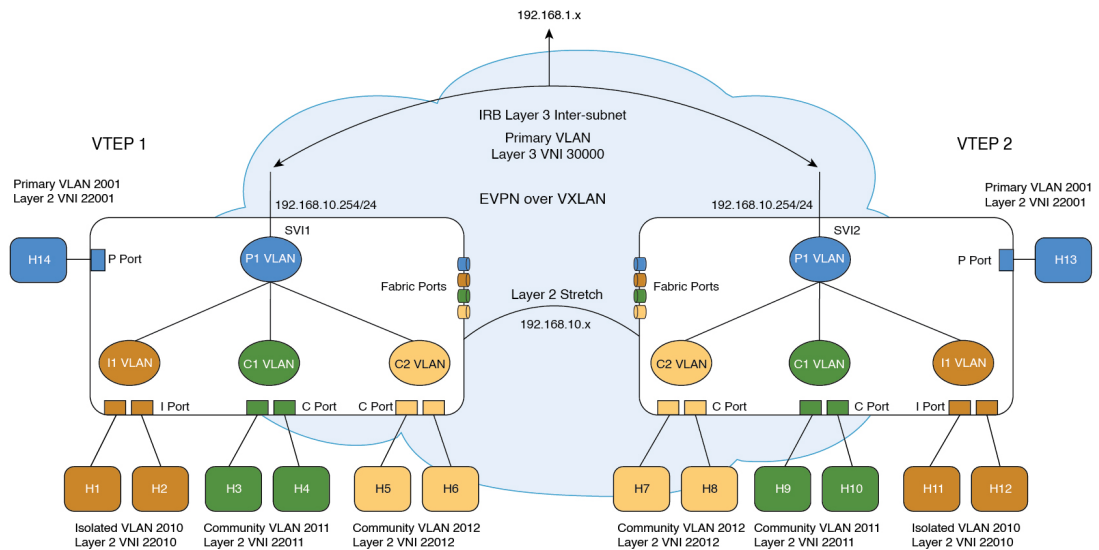
Figure 54: PVLAN Extension in a BGP EVPN VXLAN Fabric
