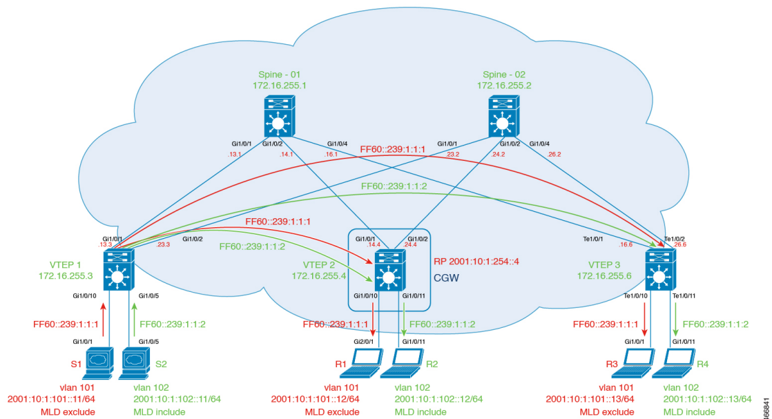
Figure 66: Topology for Optimized Layer 2 Overlay Multicast with Ingress Replication for IPv6 Traffic
