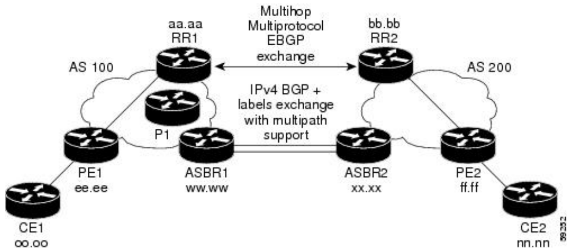
Figure 31: Distributing IPv4 Routes and MPLS Labels Between MPLS VPN Service Providers
