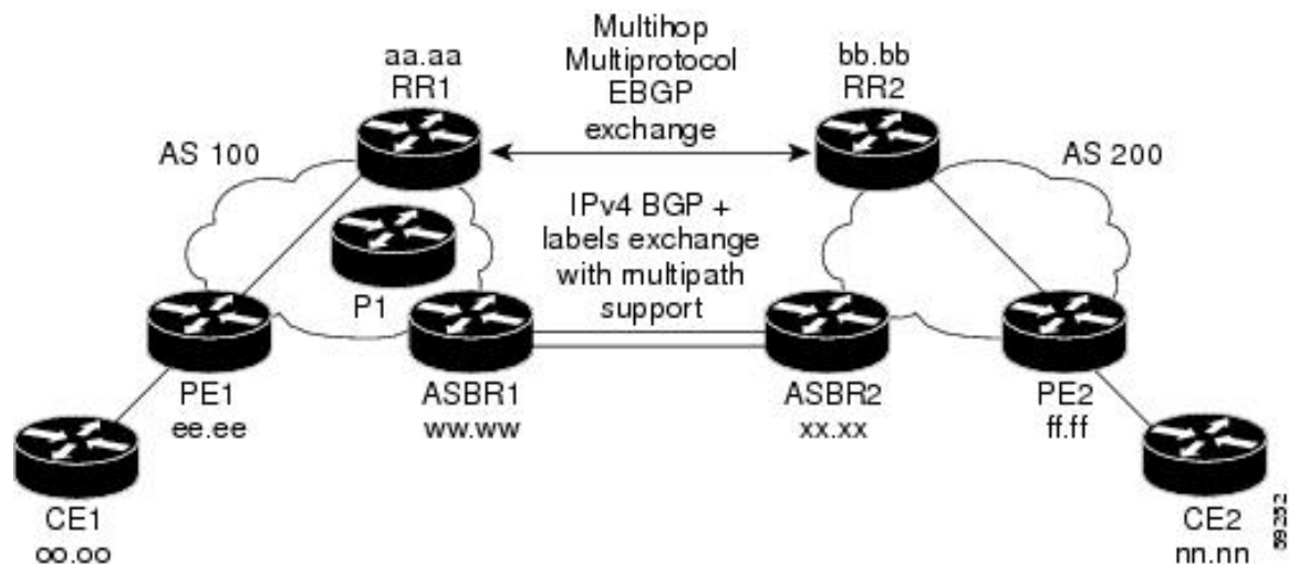
Figure 29: Configuring Two VPN Service Providers to Exchange IPv4 Routes and MPLS Labels
