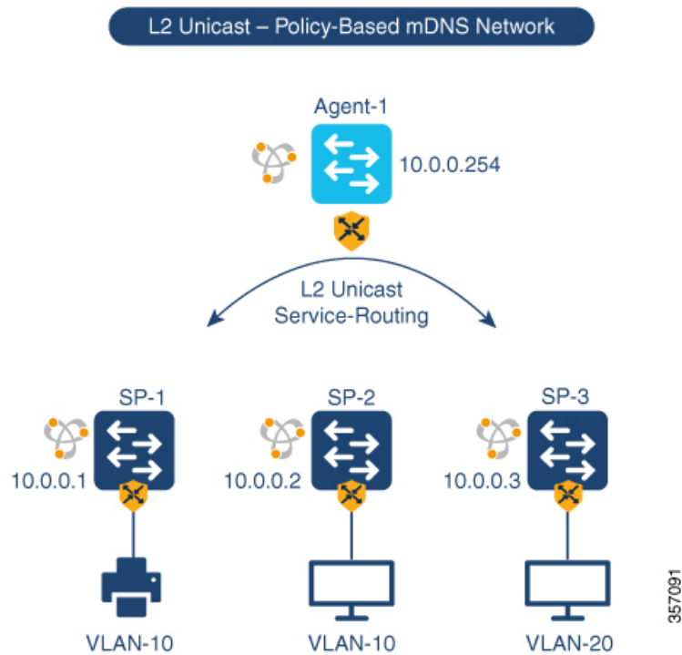
Figure 15: Unicast Mode Service-Routing for a Multilayer Network
