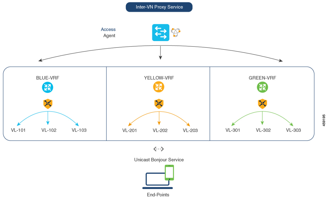
Figure 24: Inter-VN Proxy Service
