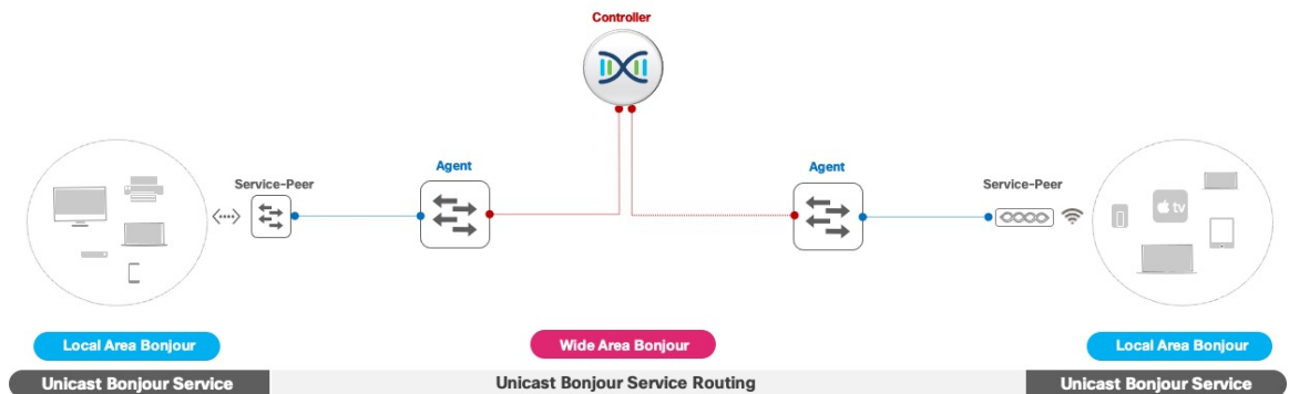
Figure 12: Cisco Wide Area Bonjour Domain
