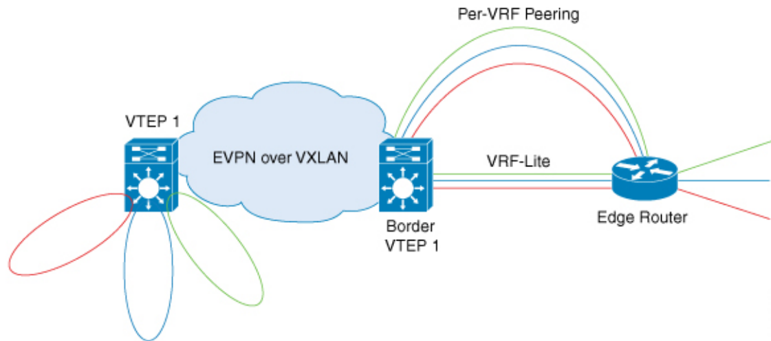
Figure 27: Layer 3 External Connectivity with VRF-Lite
