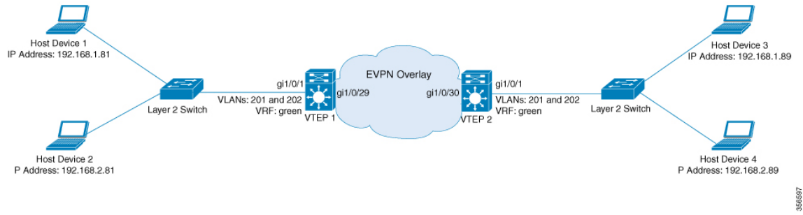
Figure 7: EVPN VXLAN Topology for IRB using Distributed Anycast Gateway
