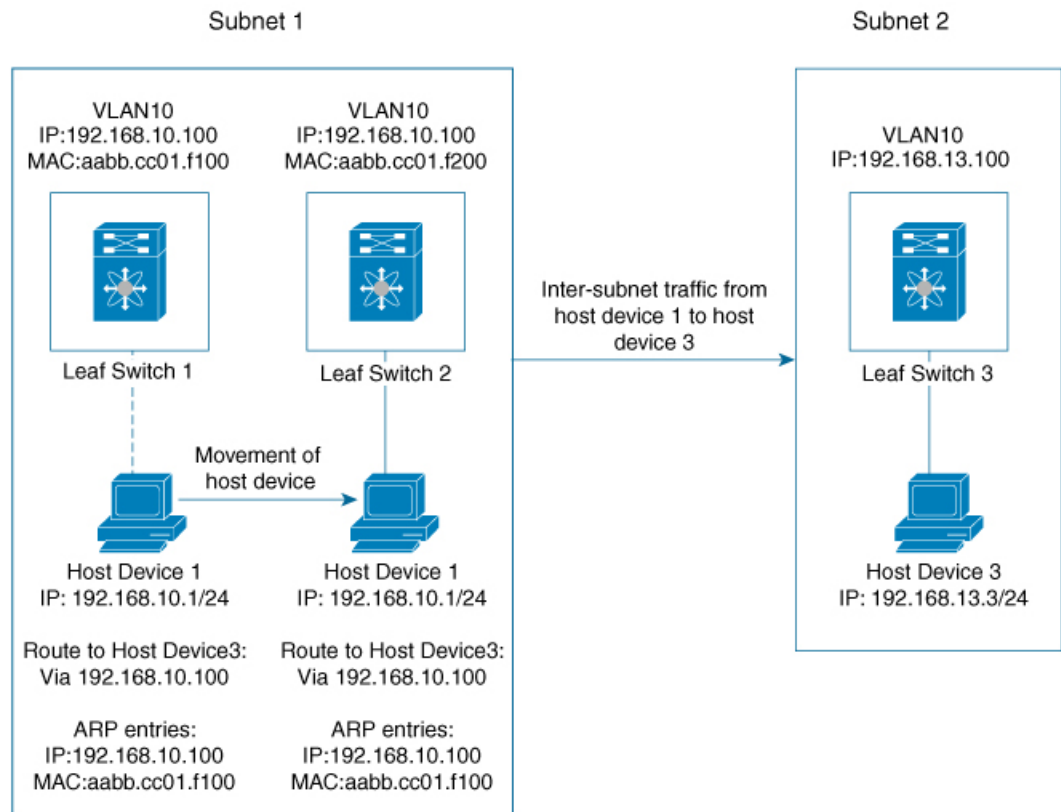
Figure 5: Distributed Gateway Topology
