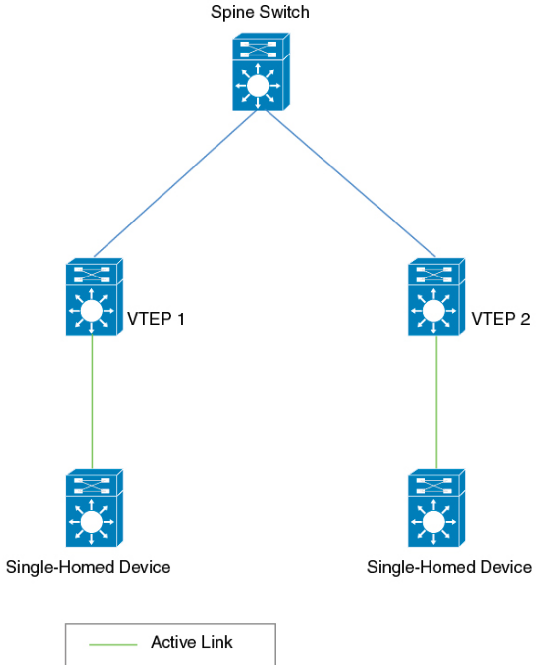
Figure 34: Single-Homed Topology
