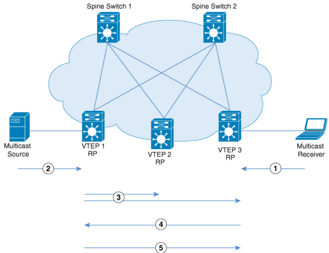
Figure 19: PIM Sparse Mode with Anycast RP
