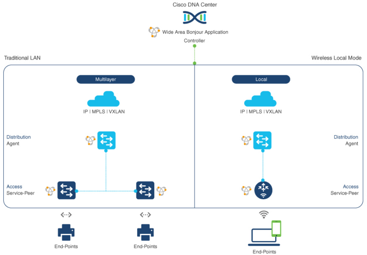
Figure 53: Enterprise Traditional LAN Network Design
