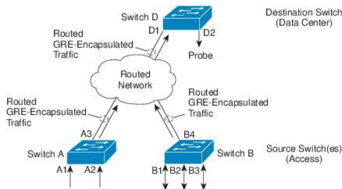
Figure 10: ERSPAN Configuration
