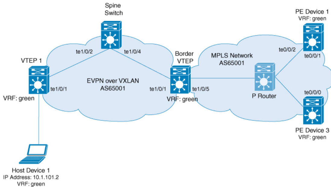
Figure 39: Layer 3 External Connectivity with MPLS Layer 3 VPN through iBGP
