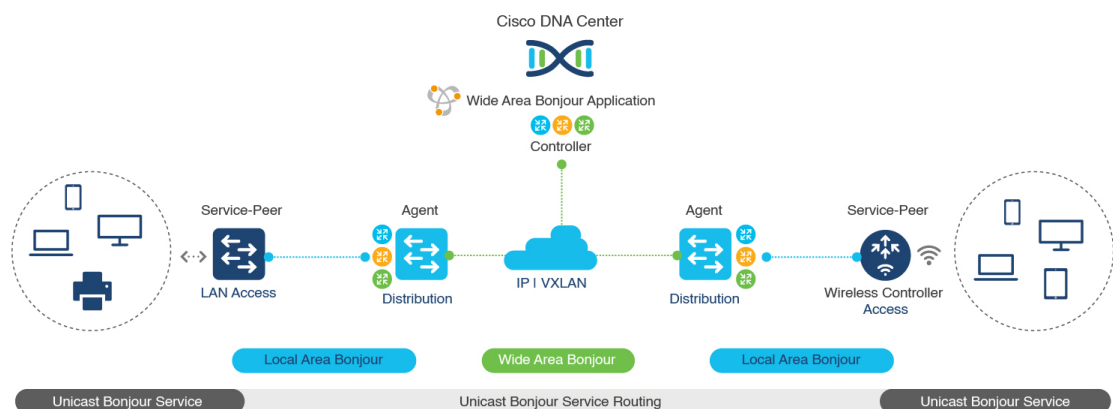
Figure 73: Overlay Bonjour Service for a BGP EVPN-Enabled Enterprise Network
