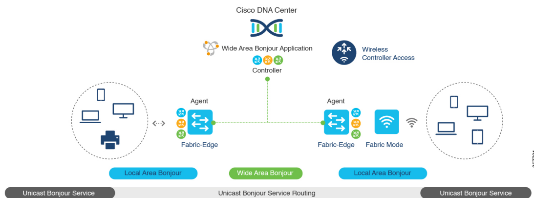
Figure 71: Cisco SD-Access Wired and Wireless Network Design
