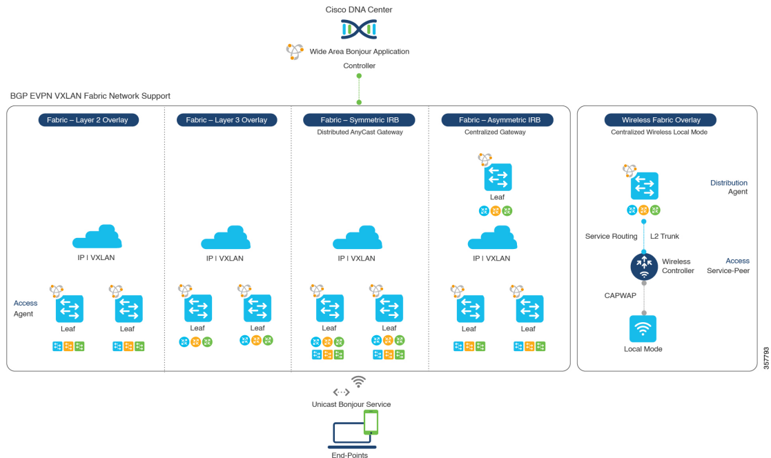
Figure 74: BGP EVPN VXLAN Wired and Wireless Design Alternatives
