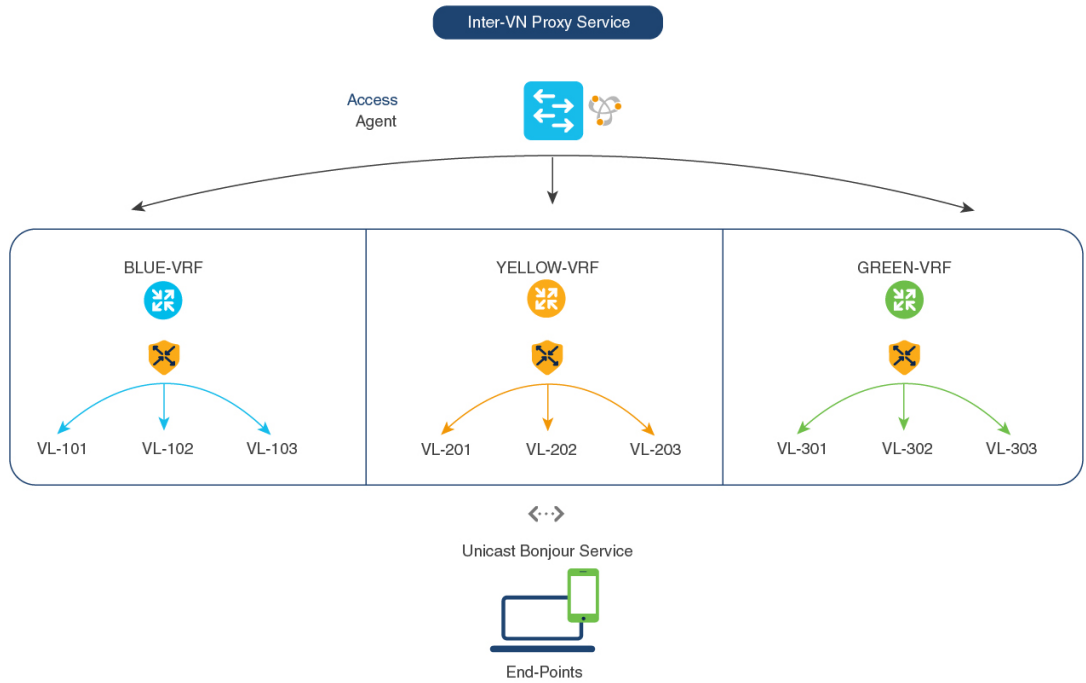
Figure 87: Inter-VN Proxy Service
