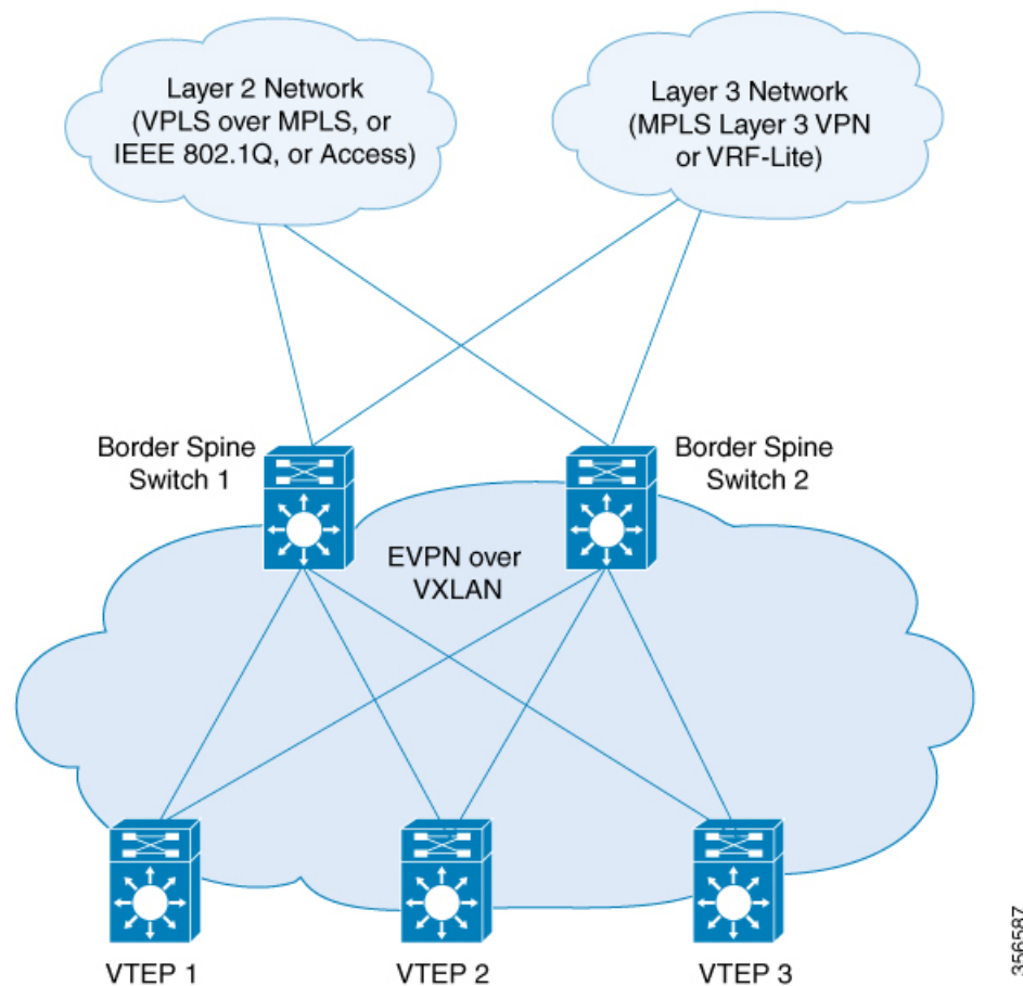
Figure 34: EVPN VXLAN External Connectivity Through a Border Spine Switch
