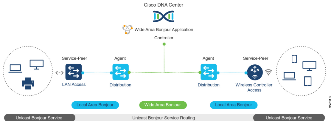
Figure 67: Cisco Wide Area Bonjour Solution Architecture
