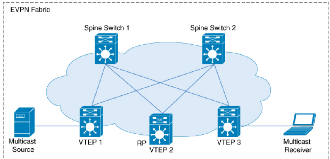
Figure 27: PIM Sparse Mode with RP Inside the BGP EVPN VXLAN Fabric
