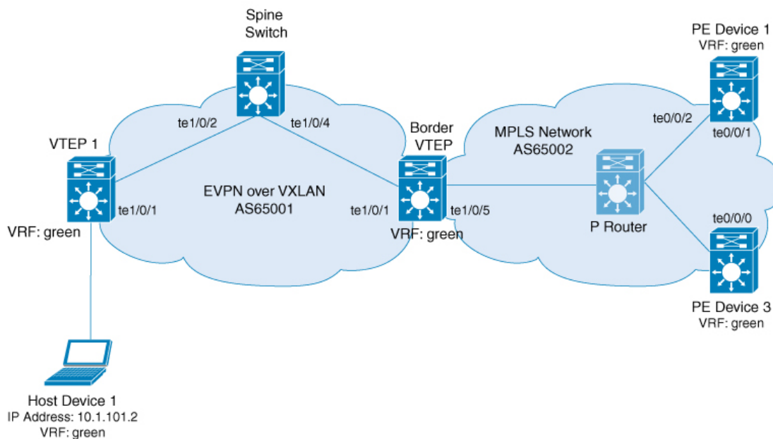
Figure 40: Layer 3 External Connectivity with MPLS Layer 3 VPN through eBGP
