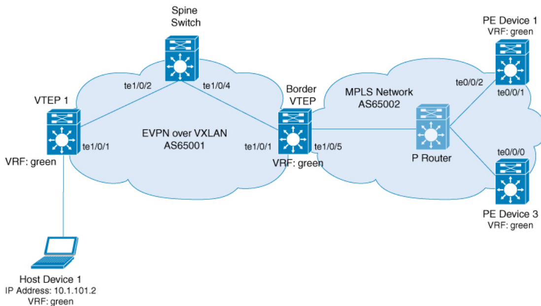
Figure 8: Layer 3 External Connectivity with MPLS Layer 3 VPN through eBGP
