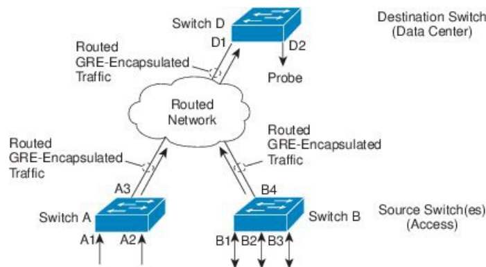
Figure 8: ERSPAN Configuration
