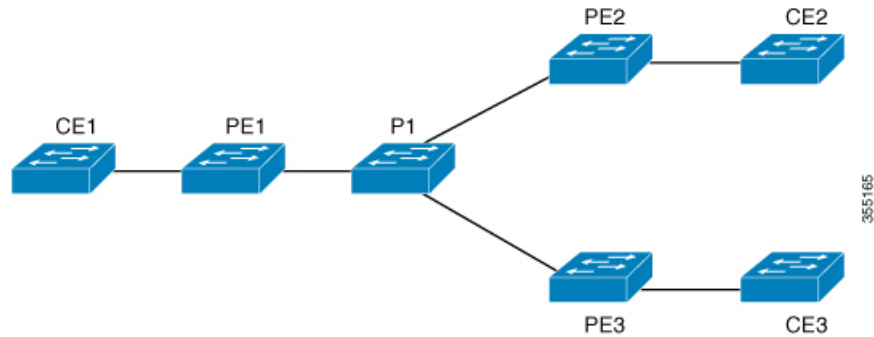
Figure 3: VPLS Topology
