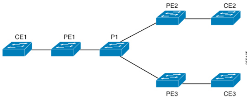
Figure 4: VPLS Topology
