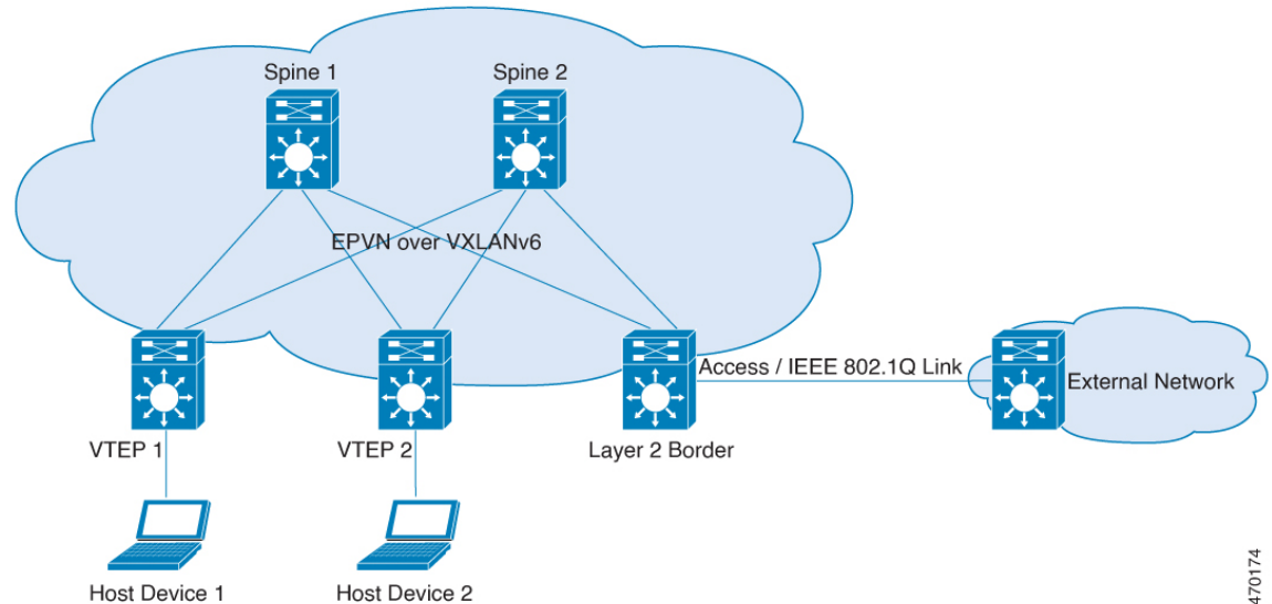
Figure 69: EVPN VXLANv6 Fabric with Layer 2 Gateway
