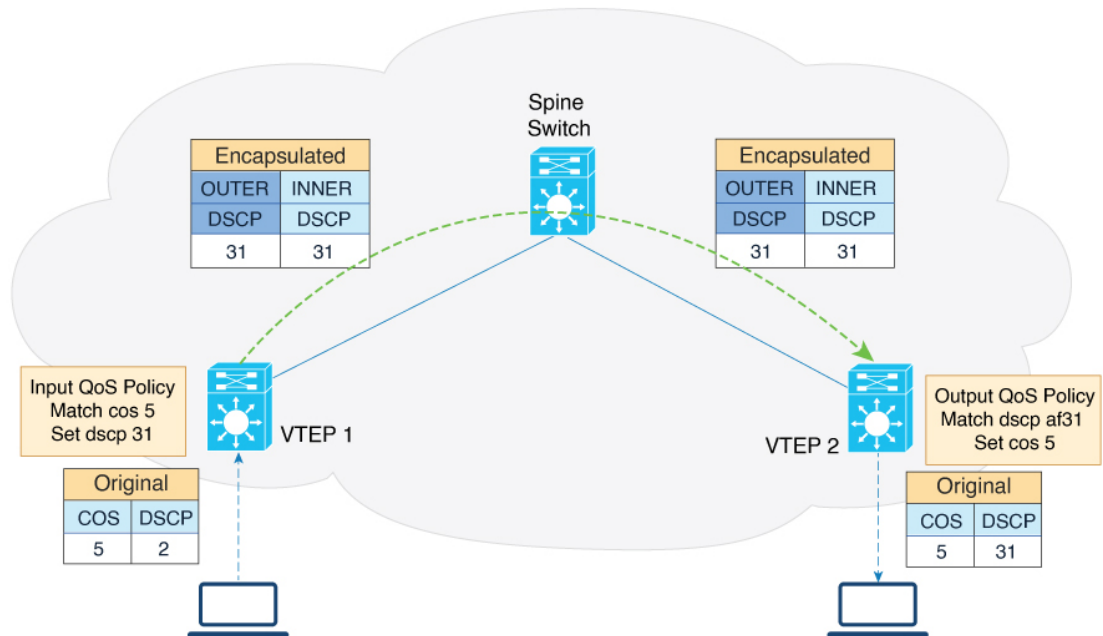
Figure 24: EVPN QoS Marking with an Input and an Output Policy
