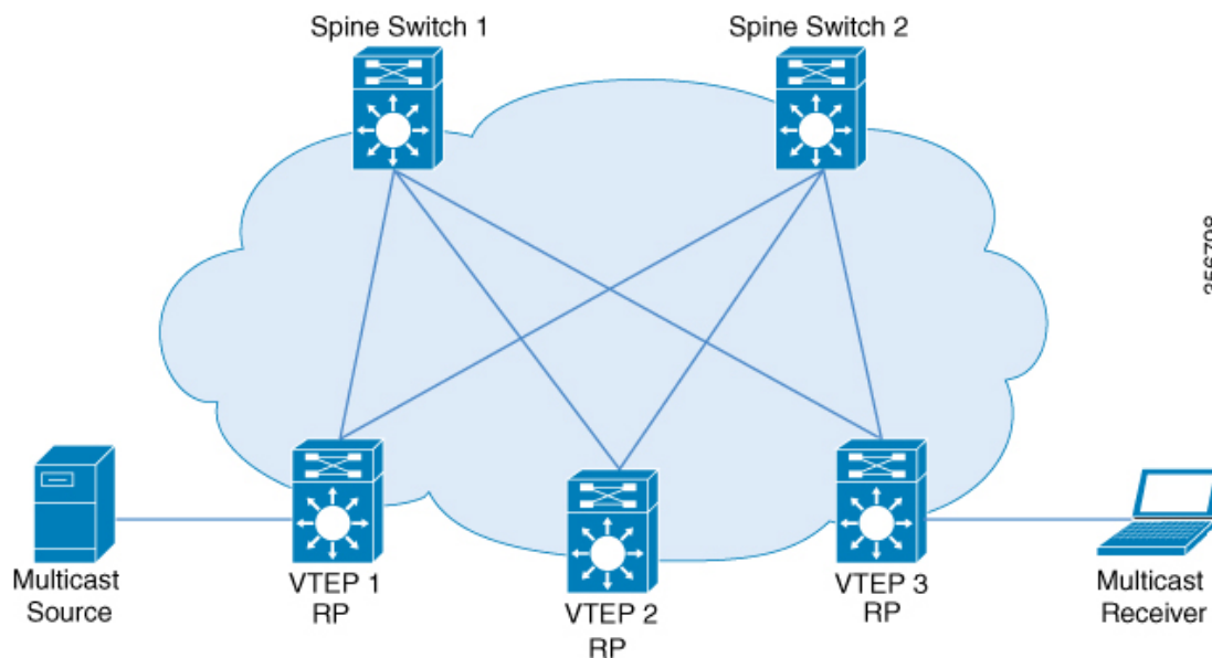
Figure 35: Anycast RP in the Overlay Network
