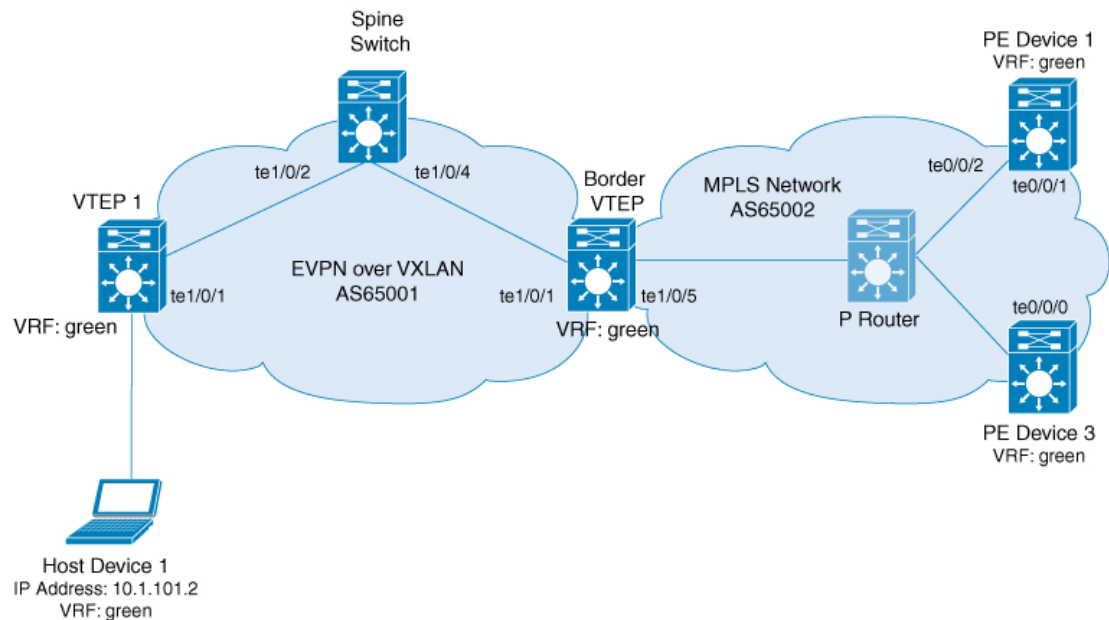
Figure 54: Layer 3 External Connectivity with MPLS Layer 3 VPN through eBGP
