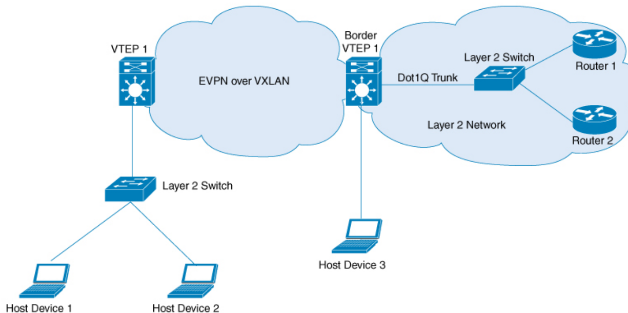
Figure 51: Layer 2 External Connectivity with IEEE 802.1Q Networks
