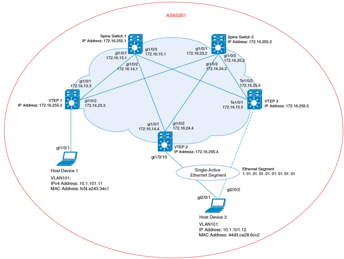
Figure 60: Dual-Homing with Single-Active Redundancy in a BGP EVPN VXLAN Fabric
