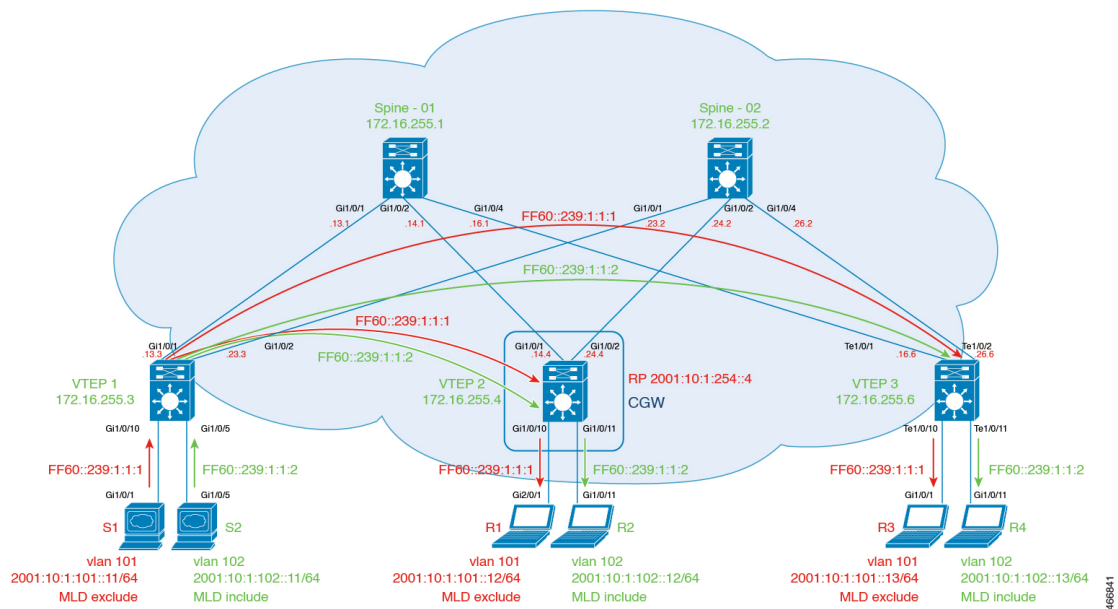
Figure 29: Topology for Optimized Layer 2 Overlay Multicast with Ingress Replication for IPv6 Traffic
