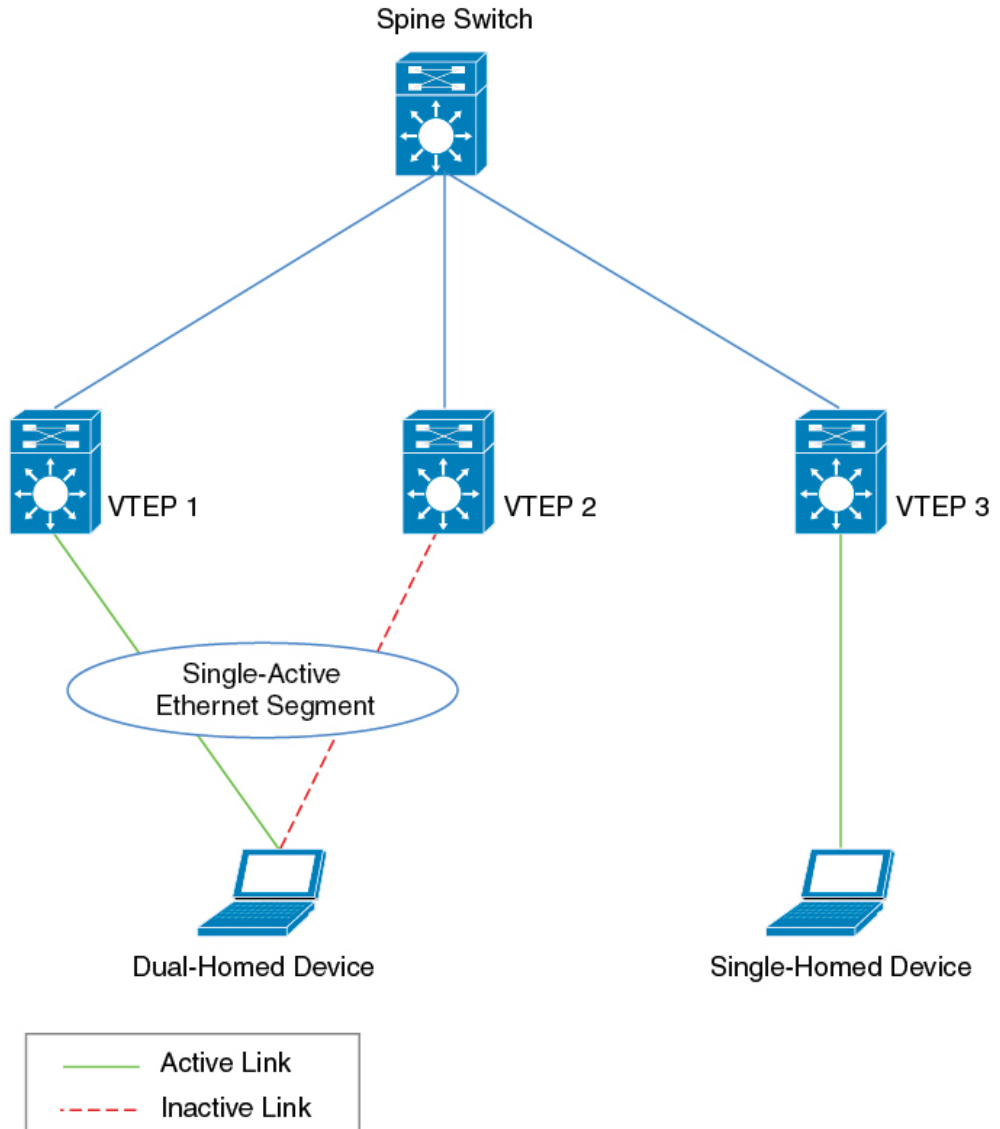
Figure 56: Dual-Homed Device Topology
