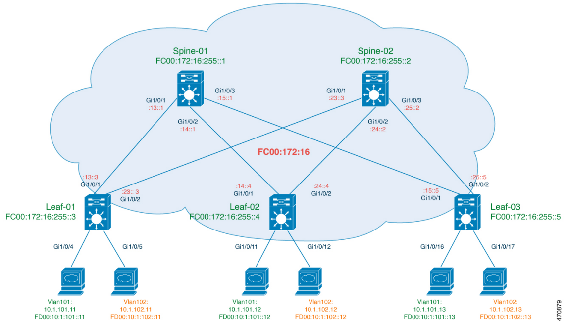
Figure 71: BGP EVPN VXLAN with IPv6 Underlay
