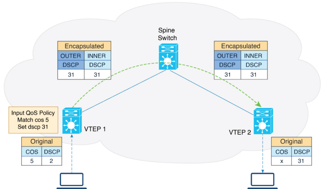
Figure 23: EVPN QoS Marking with an Input Policy
