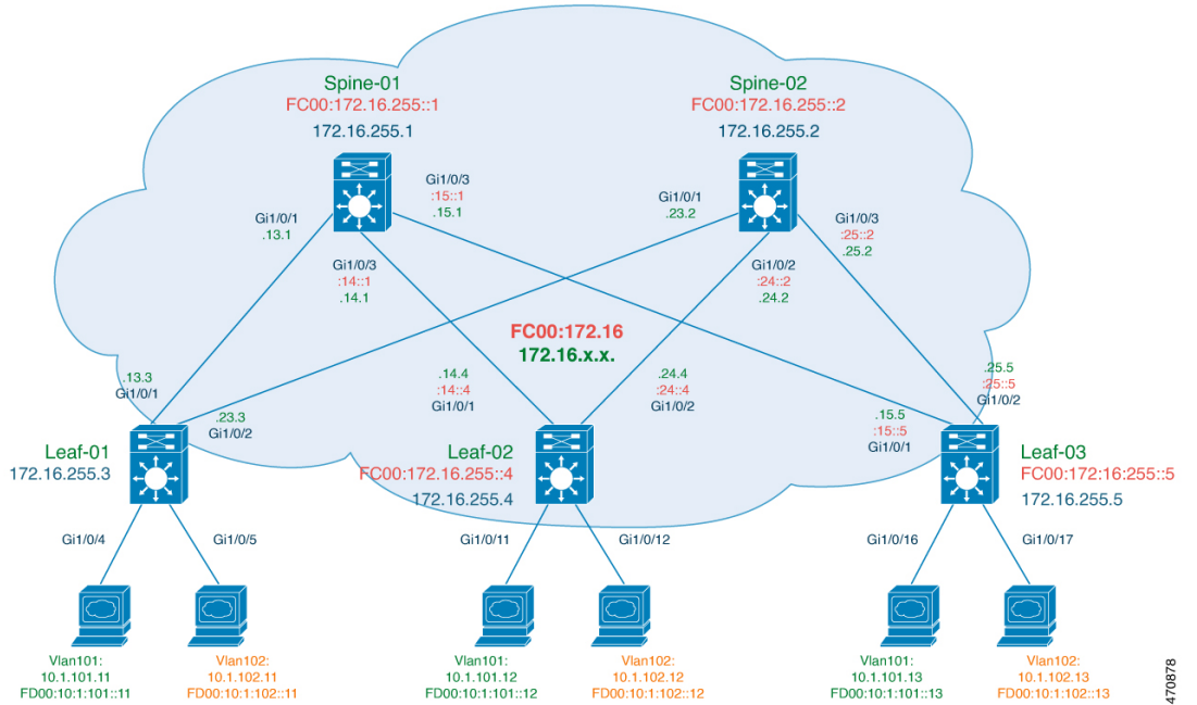
Figure 72: BGP EVPN VXLAN with a Dual Stack Underlay
