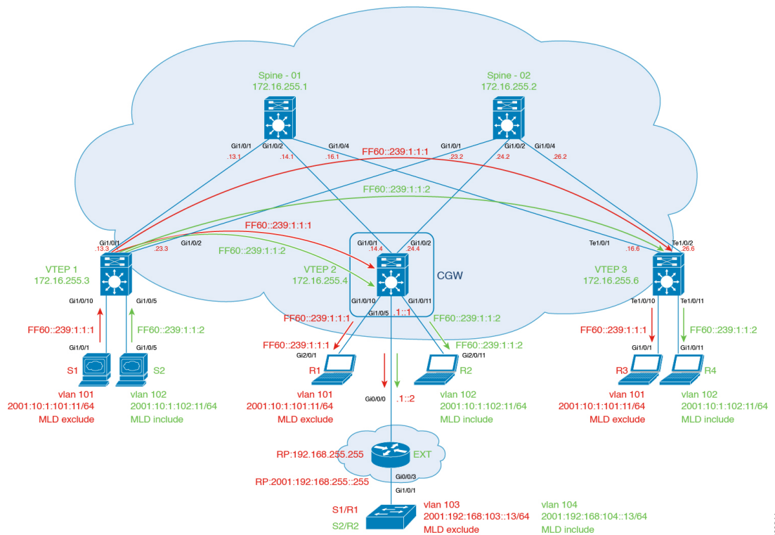
Figure 33: Topology for Optimized Layer 2 Overlay Multicast Interworking with External Network for IPv6 Traffic
