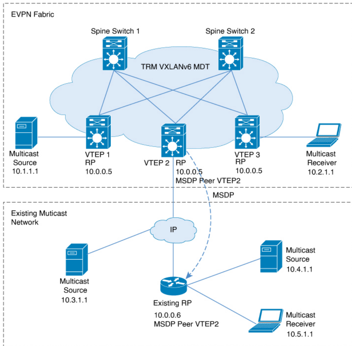
Figure 75: Anycast RP with IPv4 Overlay in an Existing Multicast Network
