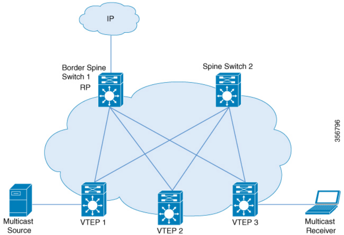
Figure 38: VTEP as an RP
