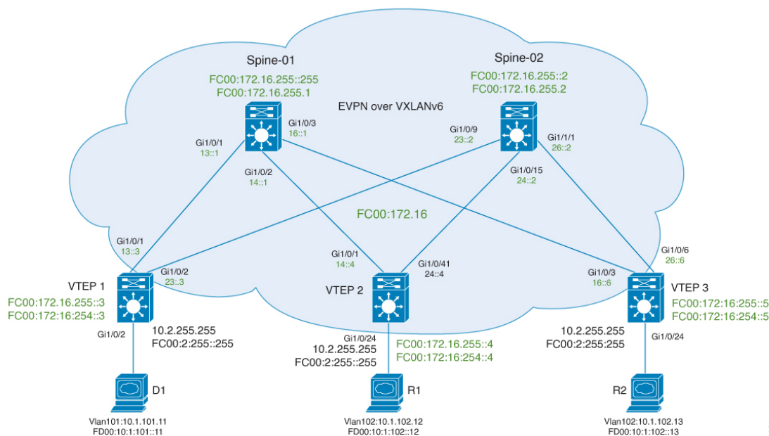
Figure 84: TRM with PIM-SM with Anycast RP over VXLANv6 Fabric
