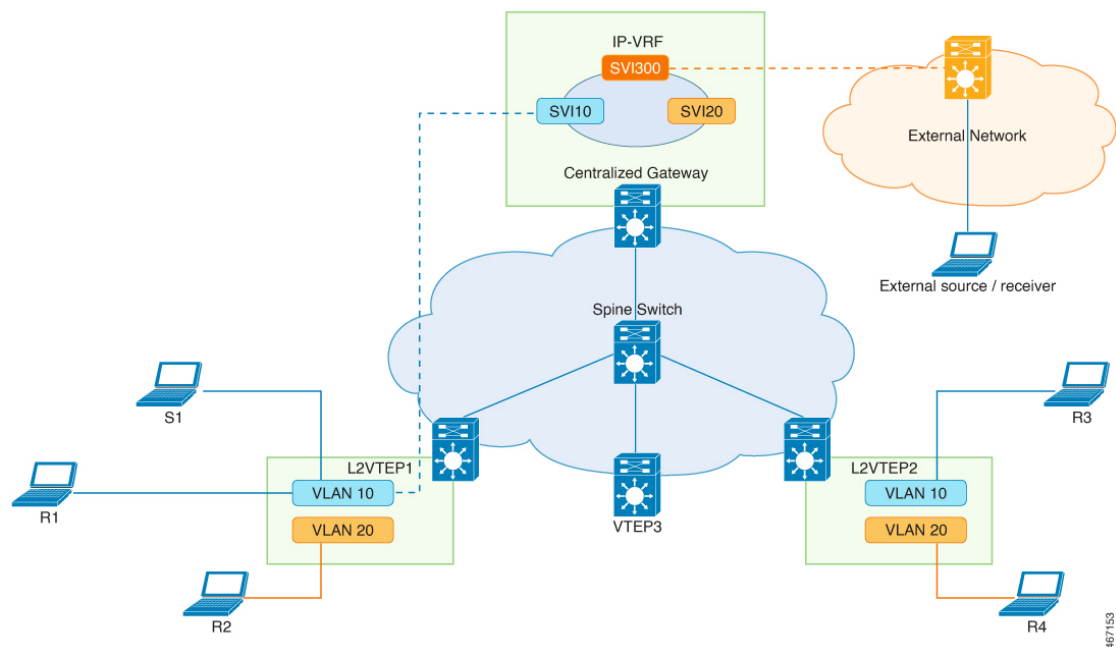
Figure 27: Topology to show Layer 2 Overlay Multicast Traffic Handoff to an External Network
