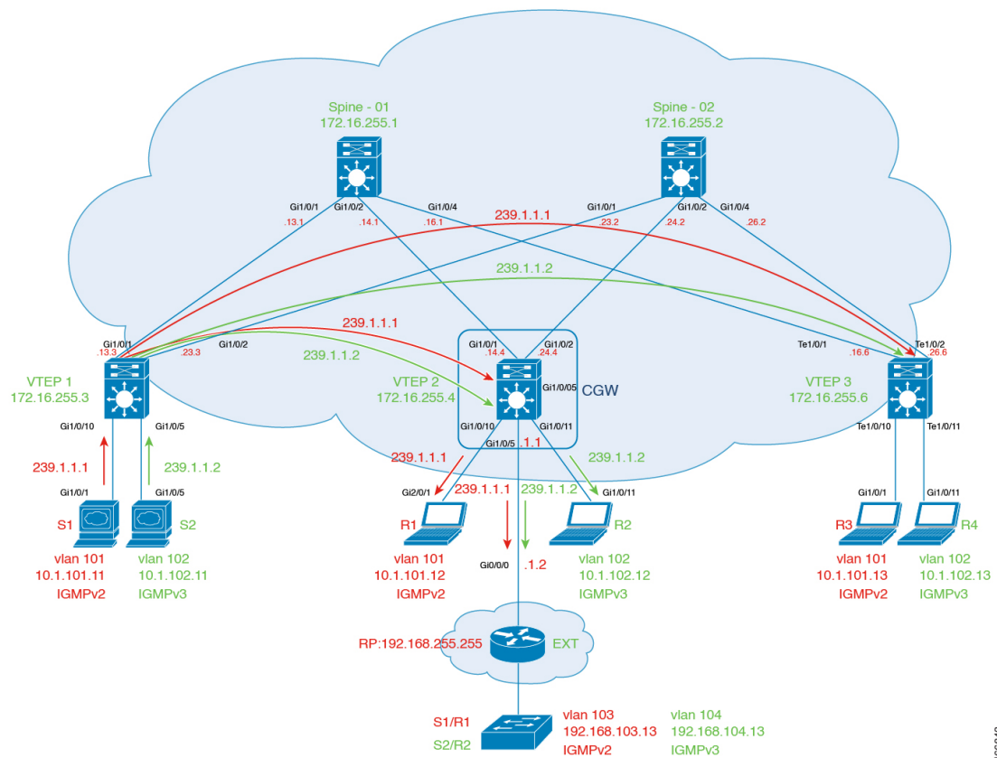
Figure 32: Topology for Optimized Layer 2 Overlay Multicast Interworking with External Network for IPv4 Traffic
