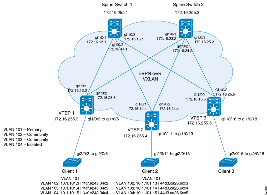
Figure 68: Private VLANs in a BGP EVPN VXLAN Fabric
