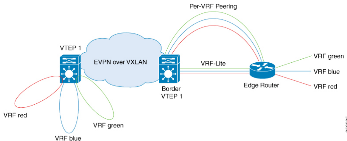
Figure 49: Layer 3 External Connectivity with VRF-Lite
