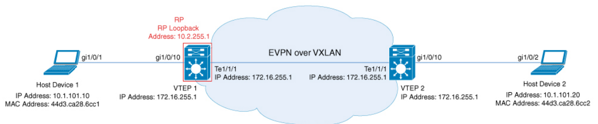
Figure 2: EVPN VXLAN Network with a Layer 2 VNI with Multicast Replication
