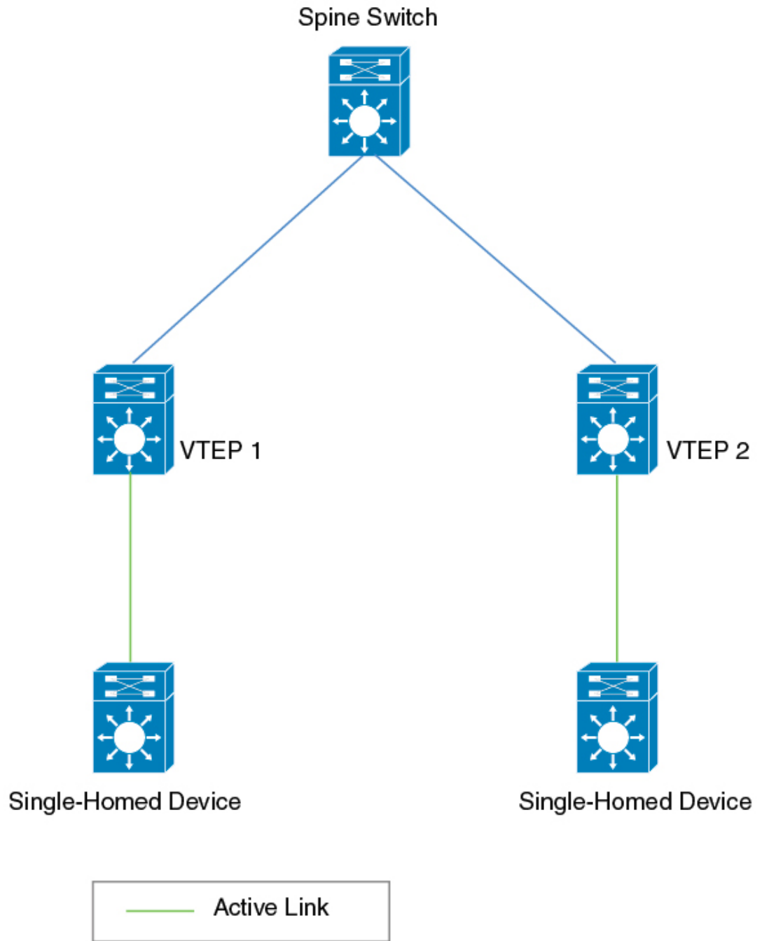
Figure 1: Single-Homed Topology
