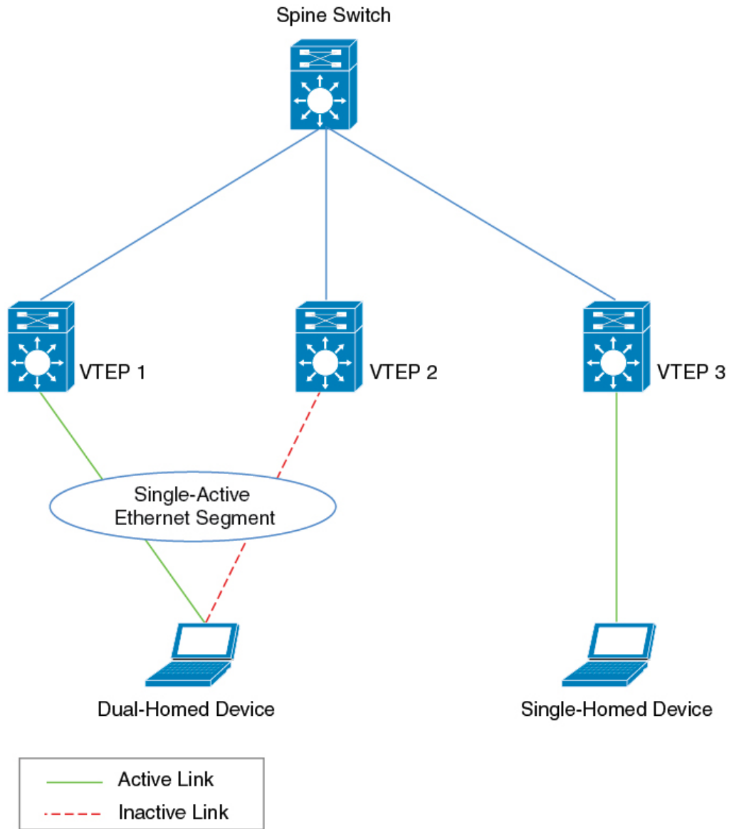
Figure 2: Dual-Homed Device Topology
