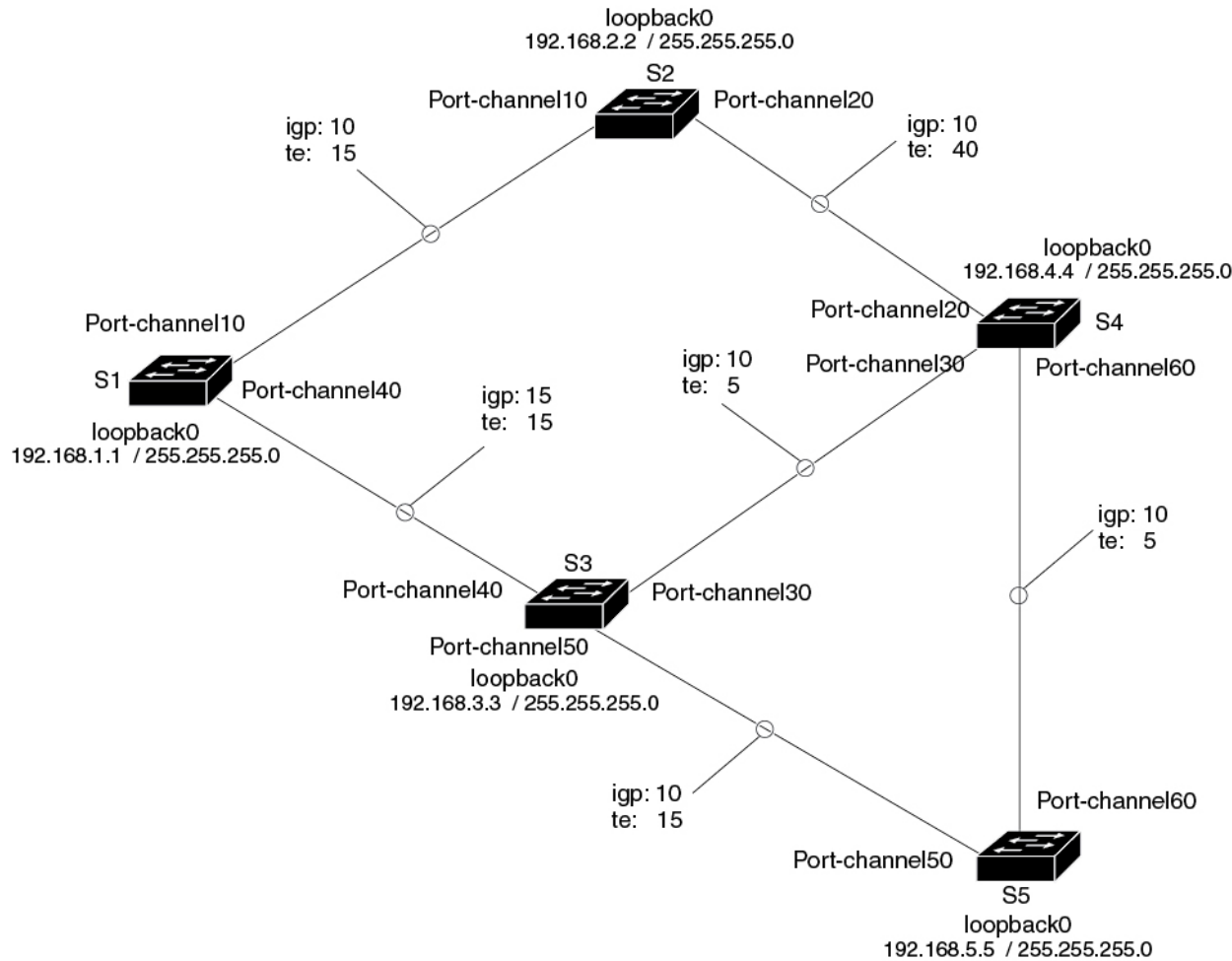
Figure 1: Network topology
