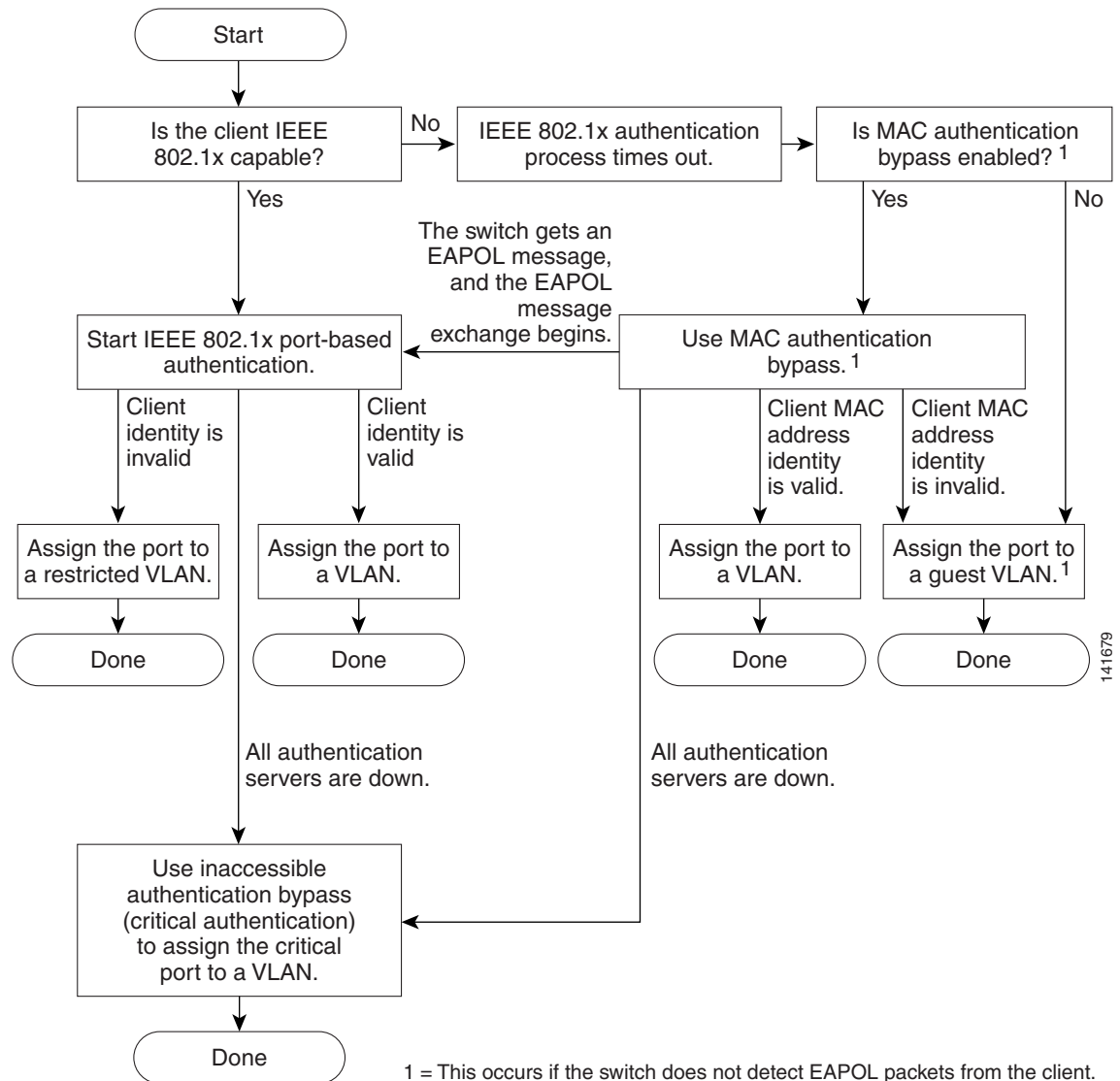
Figure 11-2 Authentication Flowchart
