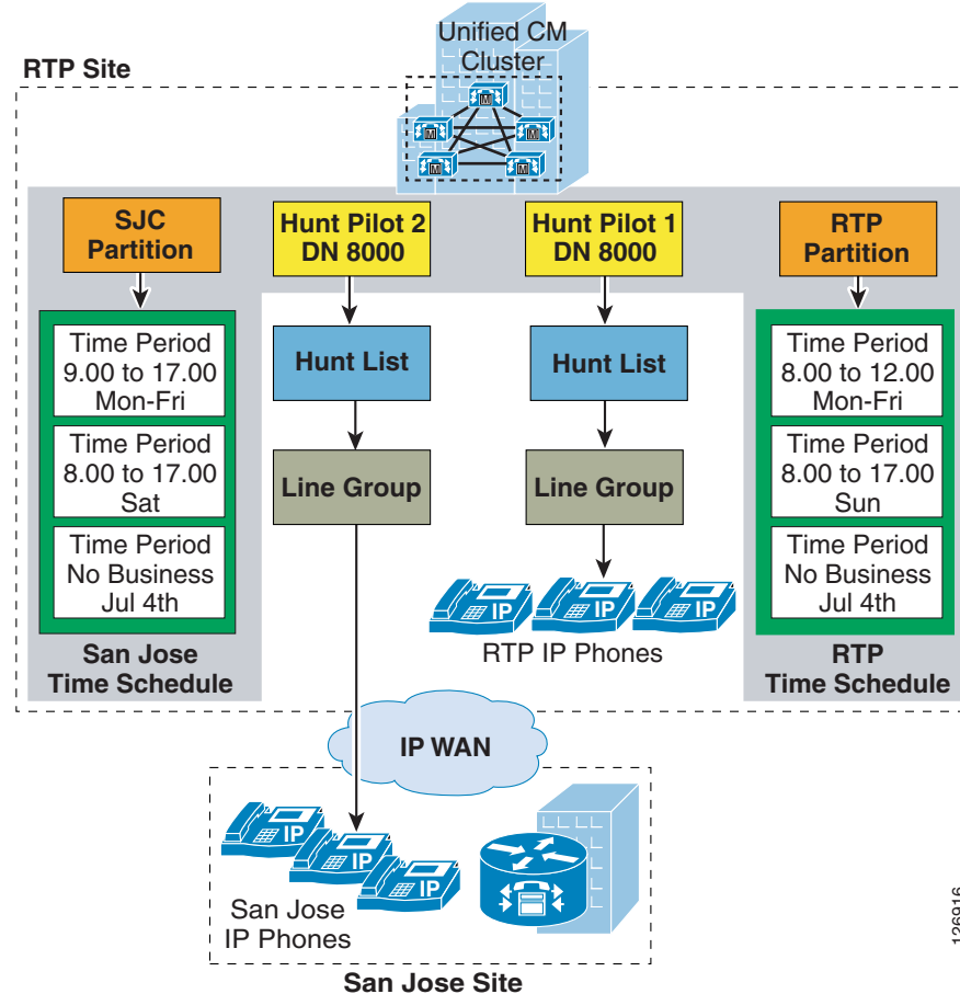
Figure 9-45 Time-of-Day Routing
