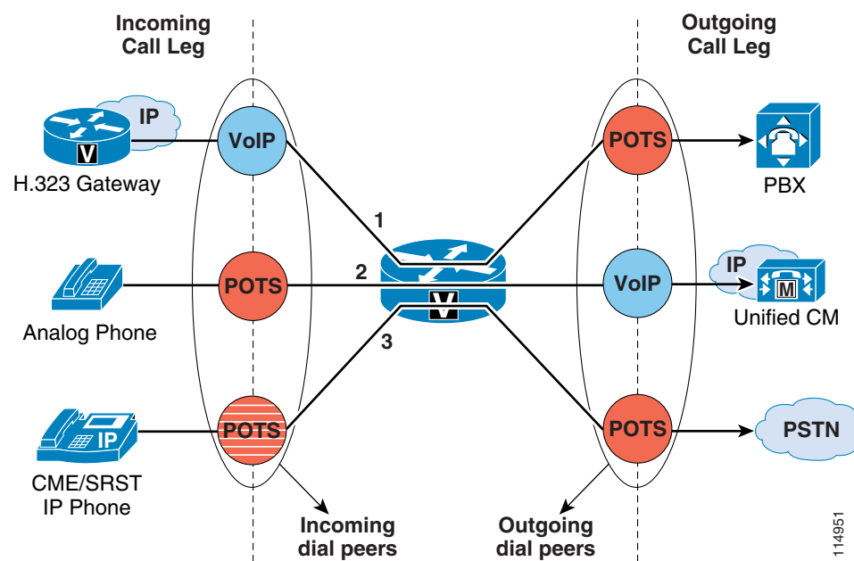
Figure 9-46 Incoming and Outgoing Dial Peers
