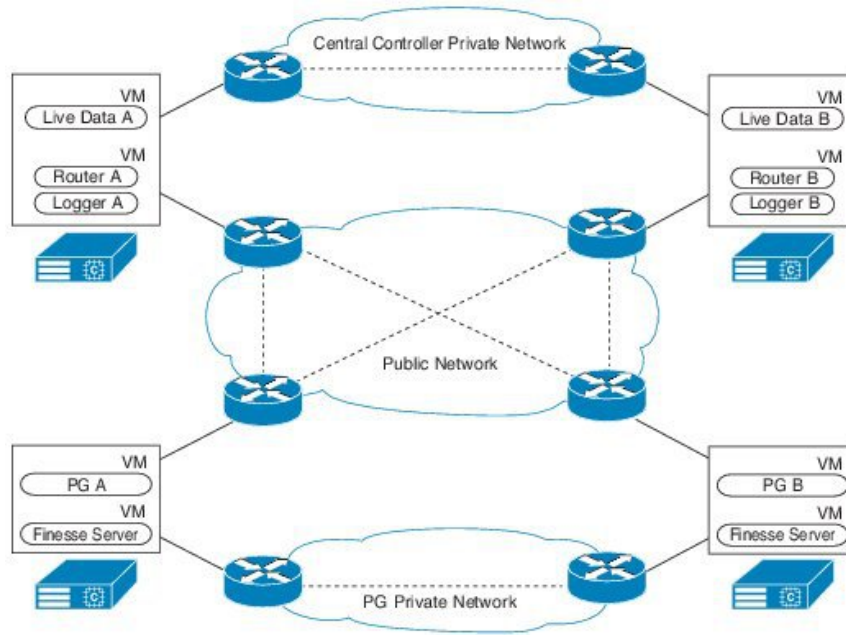
Figure 5: High Availability Design for Central Controller
