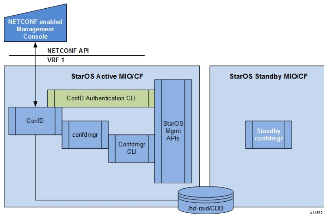
Figure 1: NETCONF System Flow
