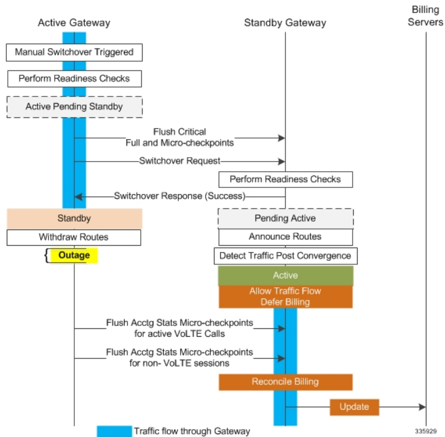
Figure 3: Call Flow: Reduce Non-VoLTE Data Outage
