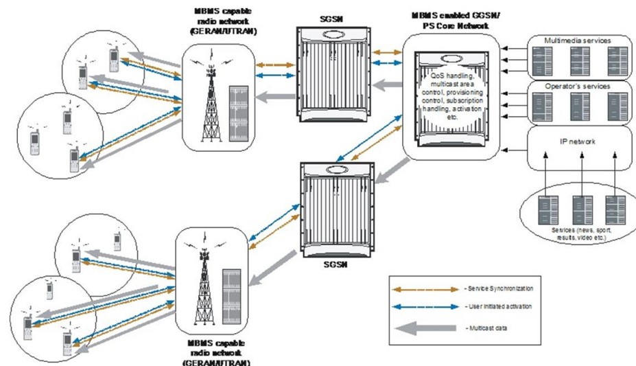
Figure 2: Basic Procedure of MBMS Multicast Mode
