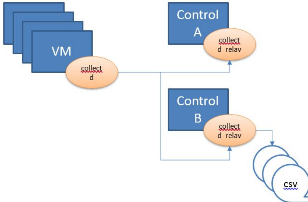
Figure 1: Architecture of CPS Bulk Statistic Collection
