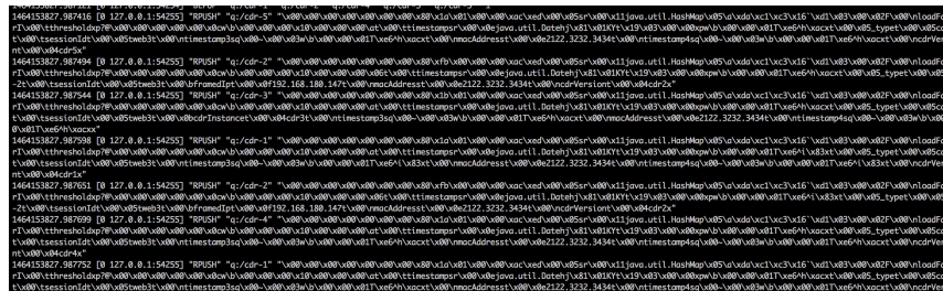
Figure 27: REDIS Output
