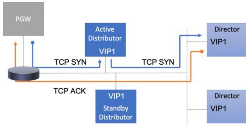
Figure 8: Direct Routing
