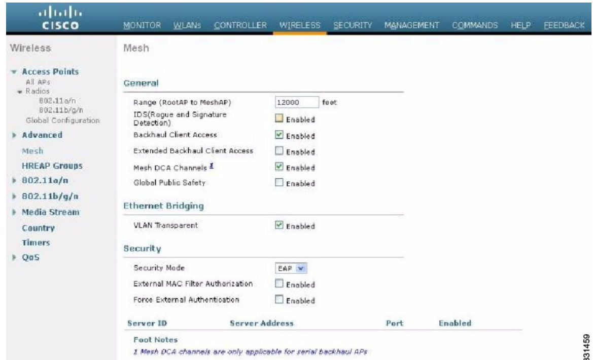
Figure 6: Configuring Backhaul Client Access using the GUI
