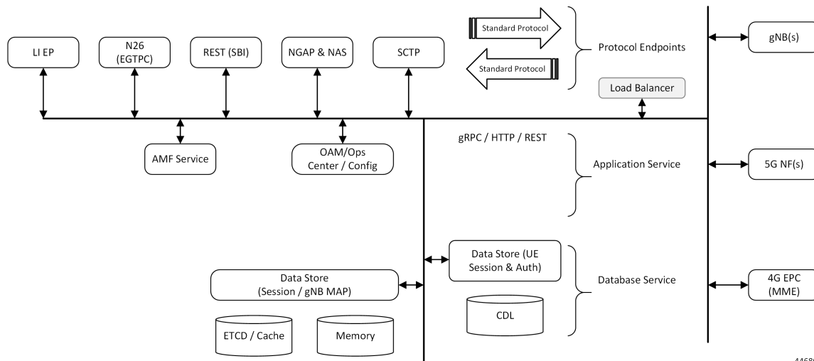
Figure 3: AMF Architecture
