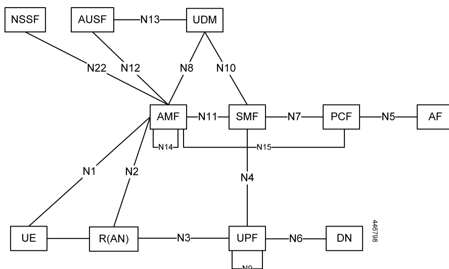
Figure 6: Interfaces
