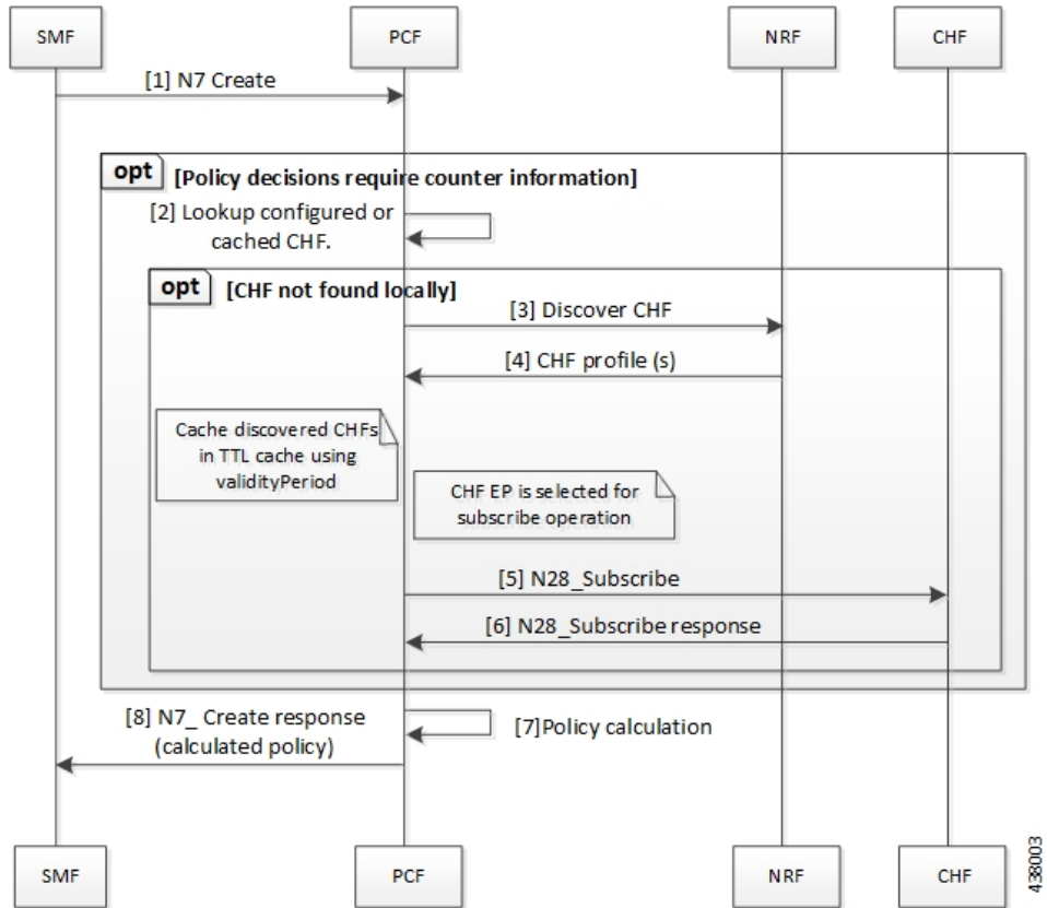
Figure 2: N28 Subscribe (N7 Create) Call Flow
